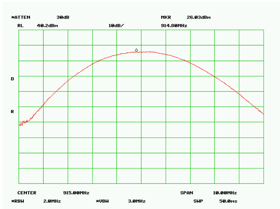
Output Power Middle Channel (Antenna Gain 5dBi)
