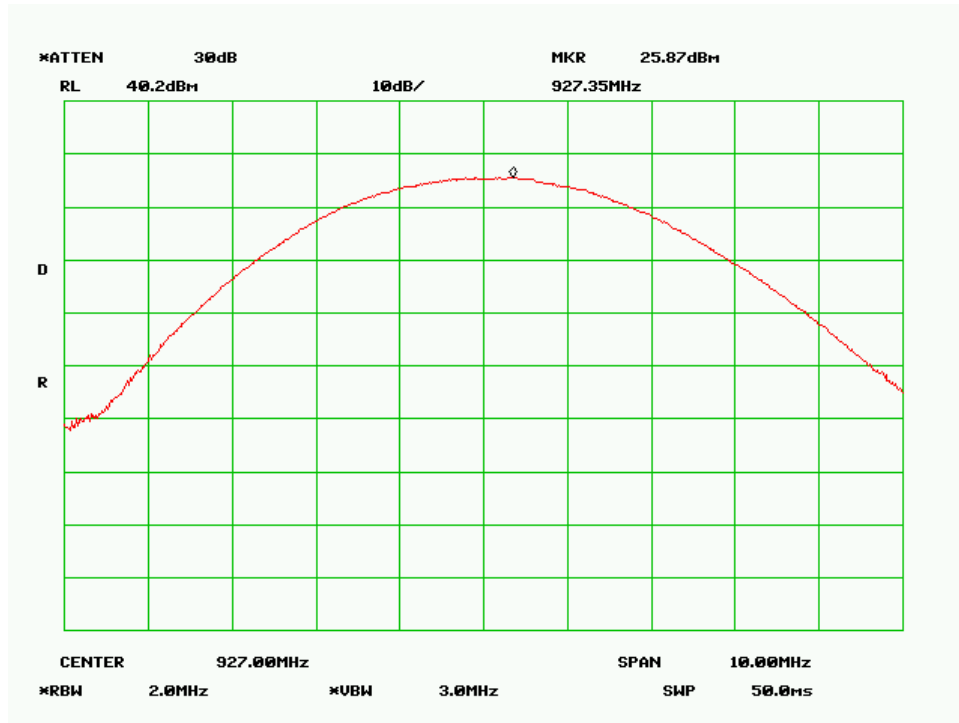
Output Power High Channel (Antenna Gain 5dBi)
