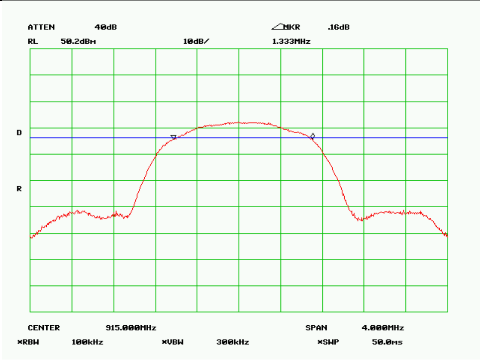
6 dB Bandwidth - Middle Channel
