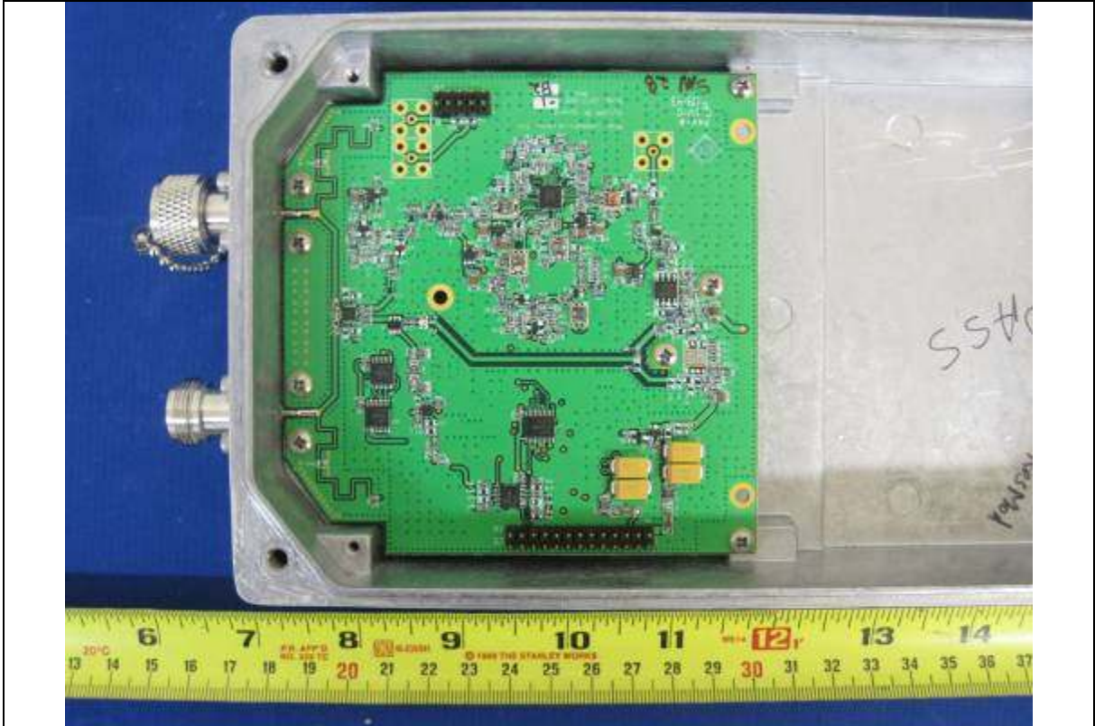
Sub-PCBA1 Solder View
