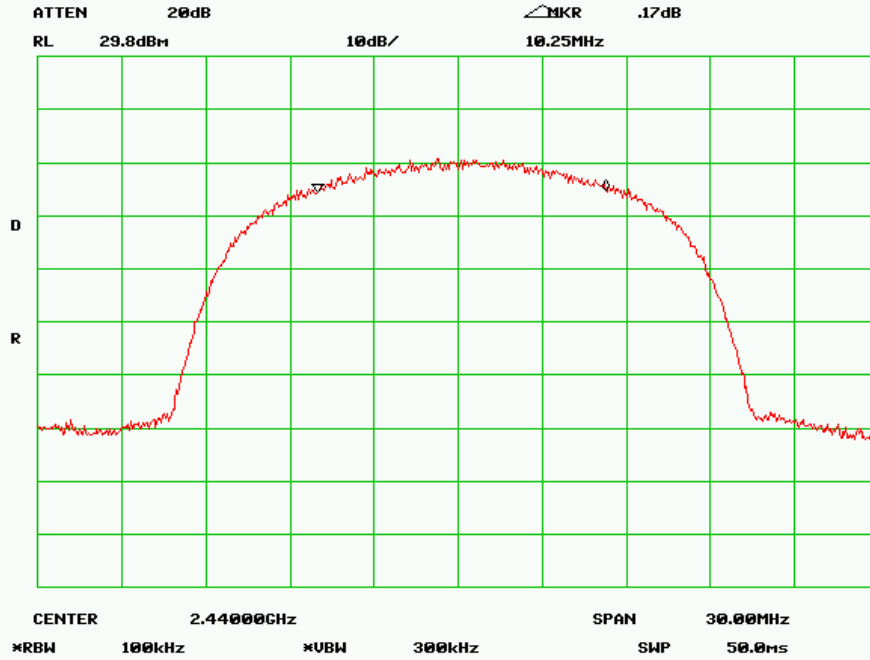
6 dB Bandwidth - Middle Channel
