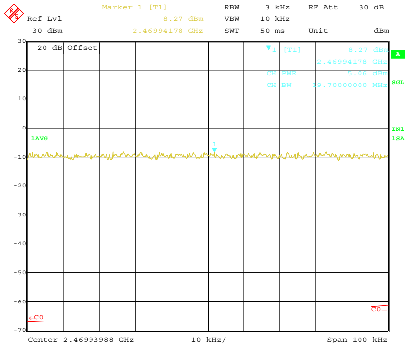
PSD High Channel(9dBi)-2
