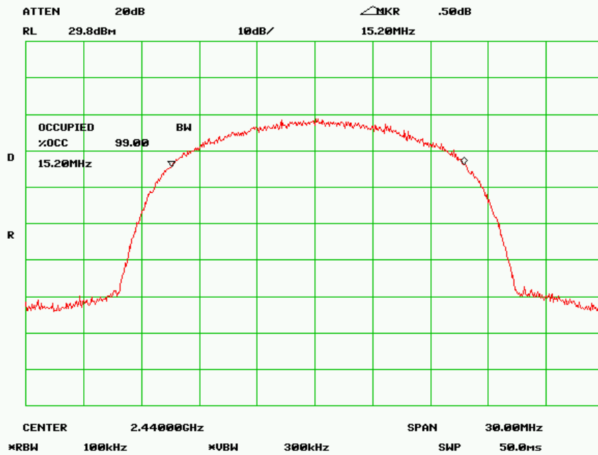
99% dB Bandwidth - Mid Channel
