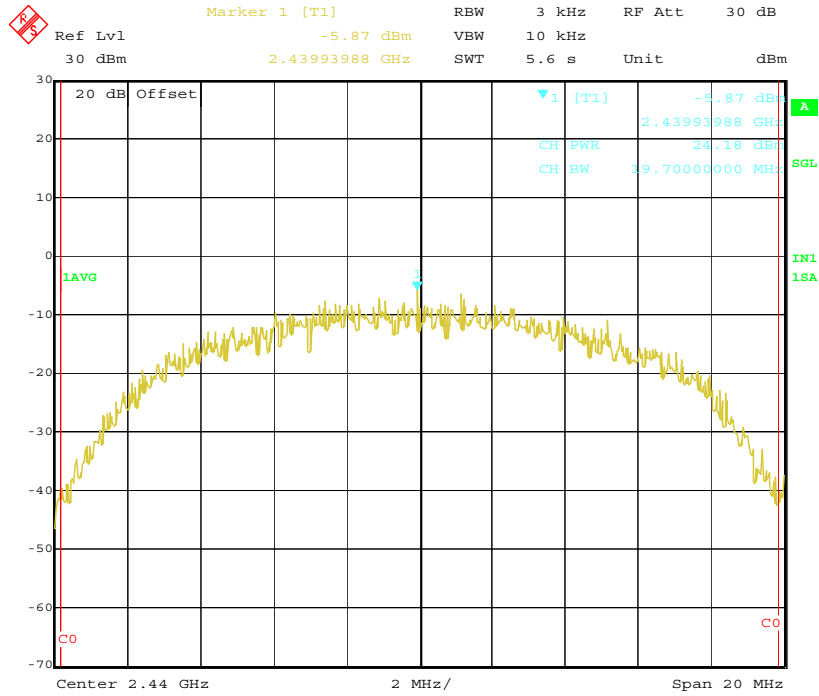
PSD Mid Channel(9dB) -1
