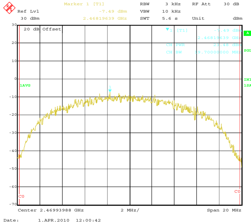
PSD High Channel(24dB)-1
