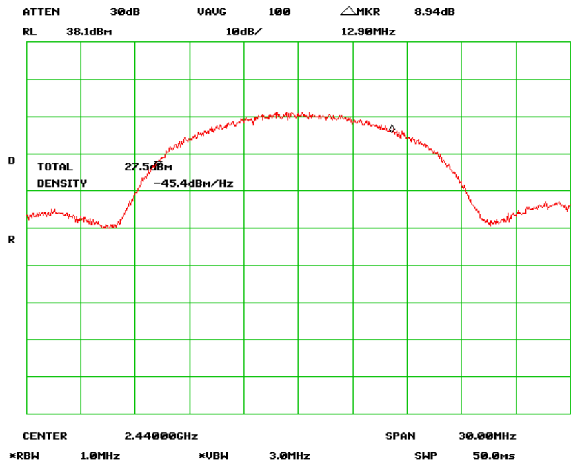
Output Power Middle Channel (Antenna Gain 9dBi)
