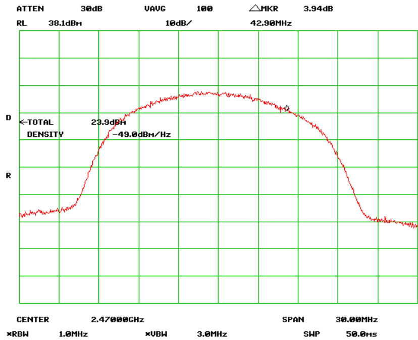
Output Power High Channel (Antenna Gain 24dBi)
