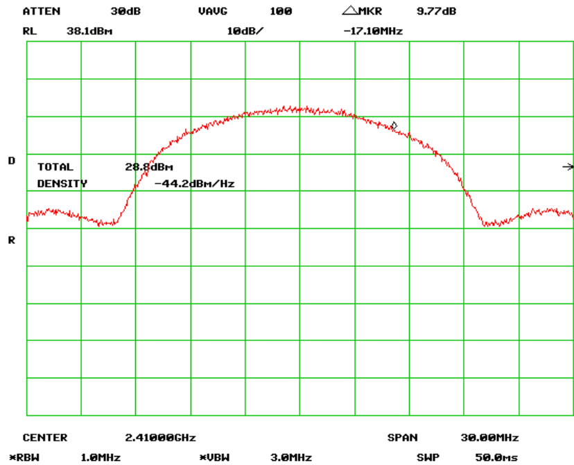
Output Power Low Channel (Antenna Gain 9dBi)
