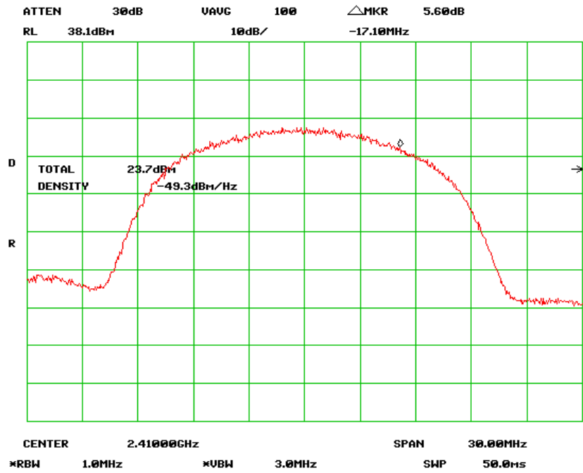
Output Power Low Channel (Antenna Gain 24dBi)
