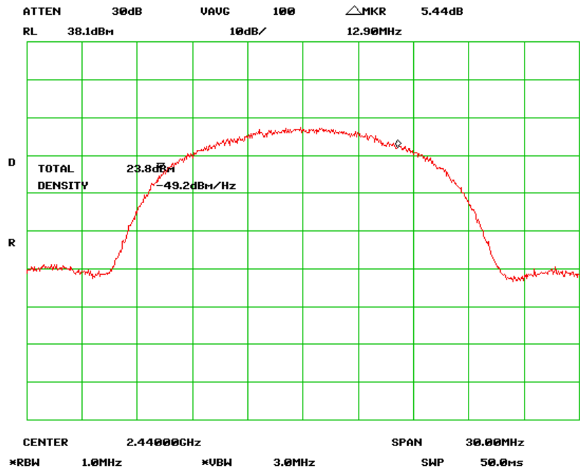
Output Power Middle Channel (Antenna Gain 24dBi)
