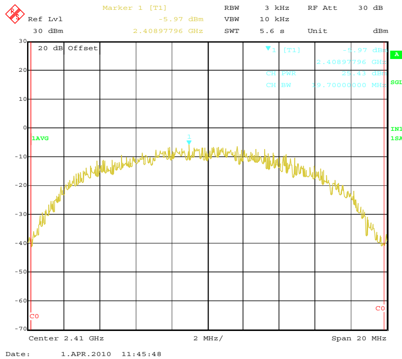
PSD Low Channel(9dB) - 1
