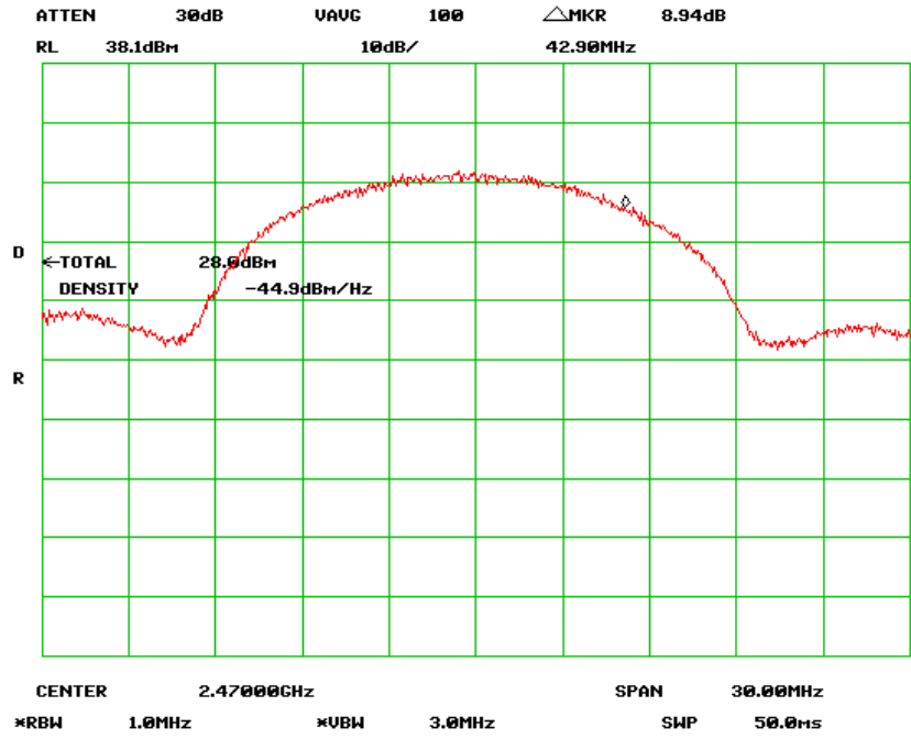
Output Power High Channel (Antenna Gain 9dBi)
