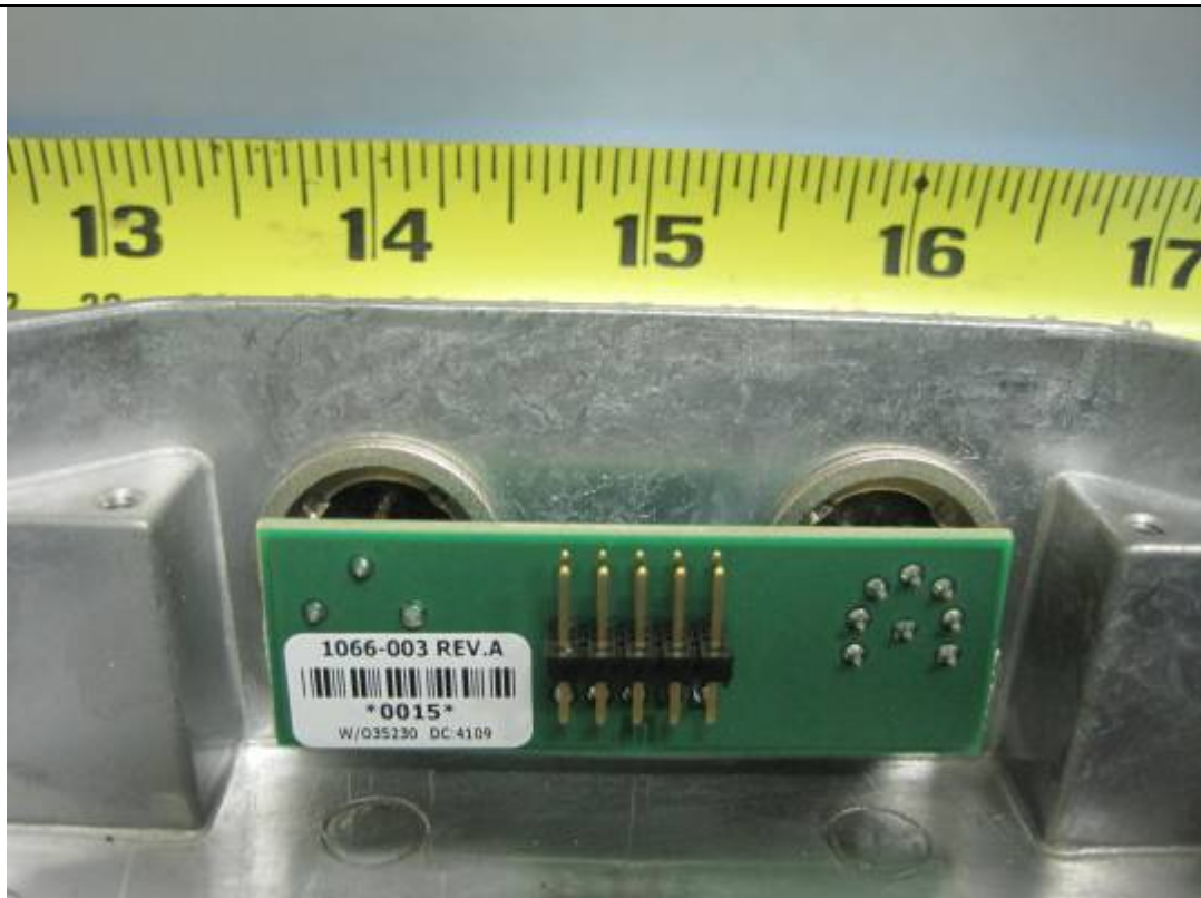
Sub-PCBA 2 Solder View
