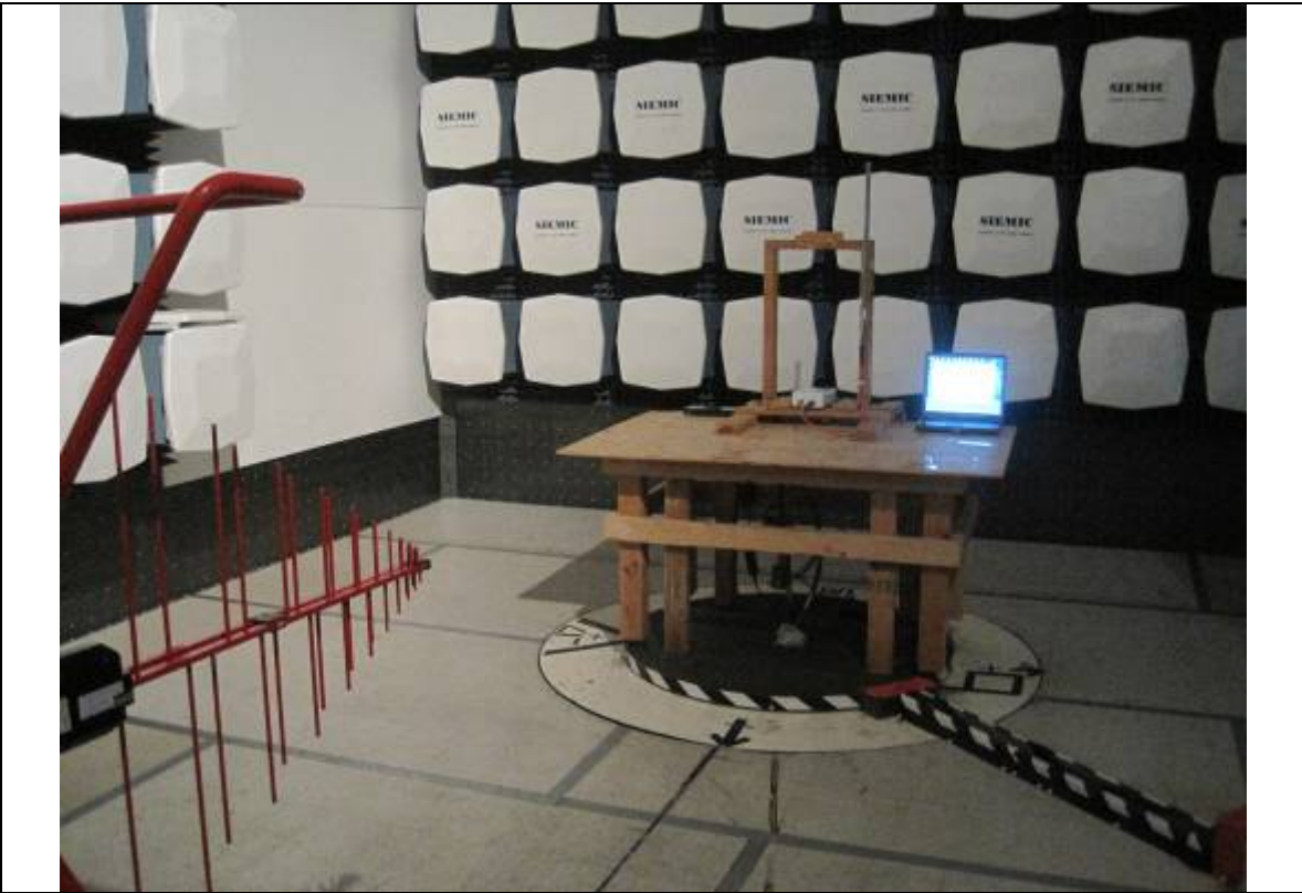
Radiated Emission Test Setup(9dBi Antenna) – Front View
