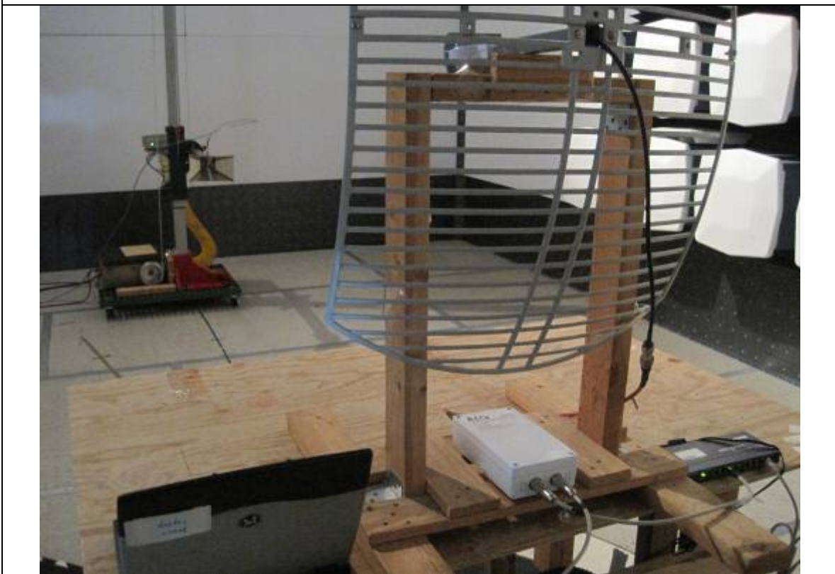
Radiated Emission Test Setup(24dBi Antenna) – Rear View
