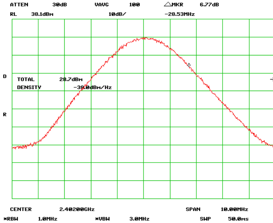
Output Power Low Channel (Antenna Gain 9dBi)
