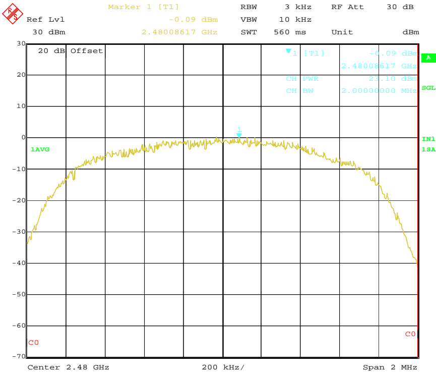
PSD High Channel(24dBi)-1
