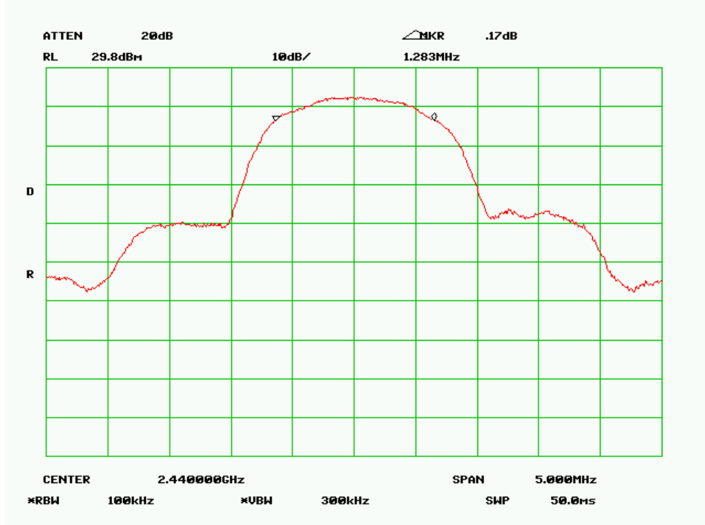
6 dB Bandwidth - Middle Channel
