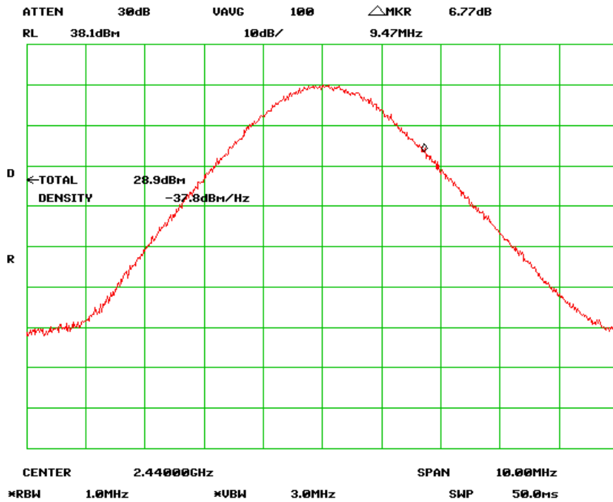
Output Power Middle Channel (Antenna Gain 9dBi)
