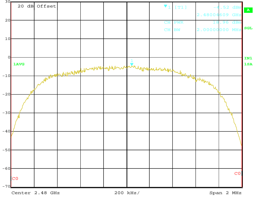
PSD High Channel(9dB)-1
