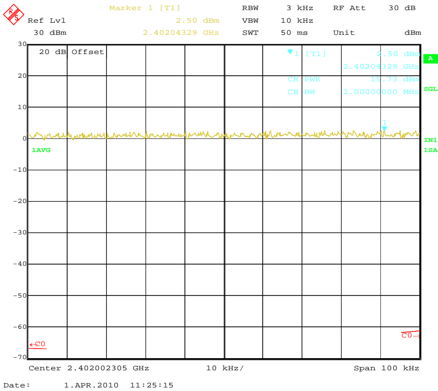
PSD Low Channel(9dBi) -2
