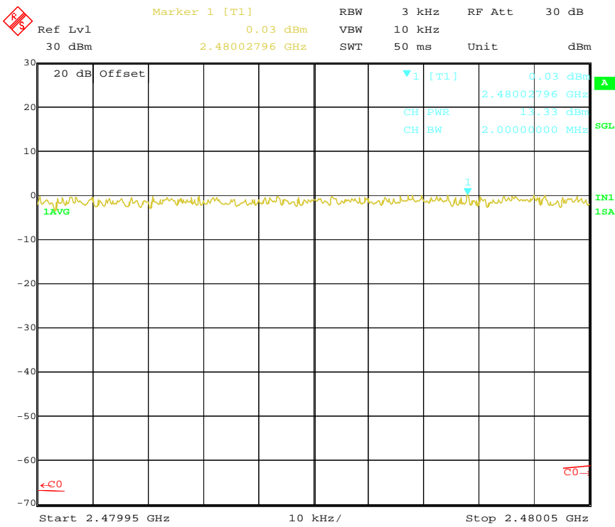
PSD High Channel(24dBi)-2
