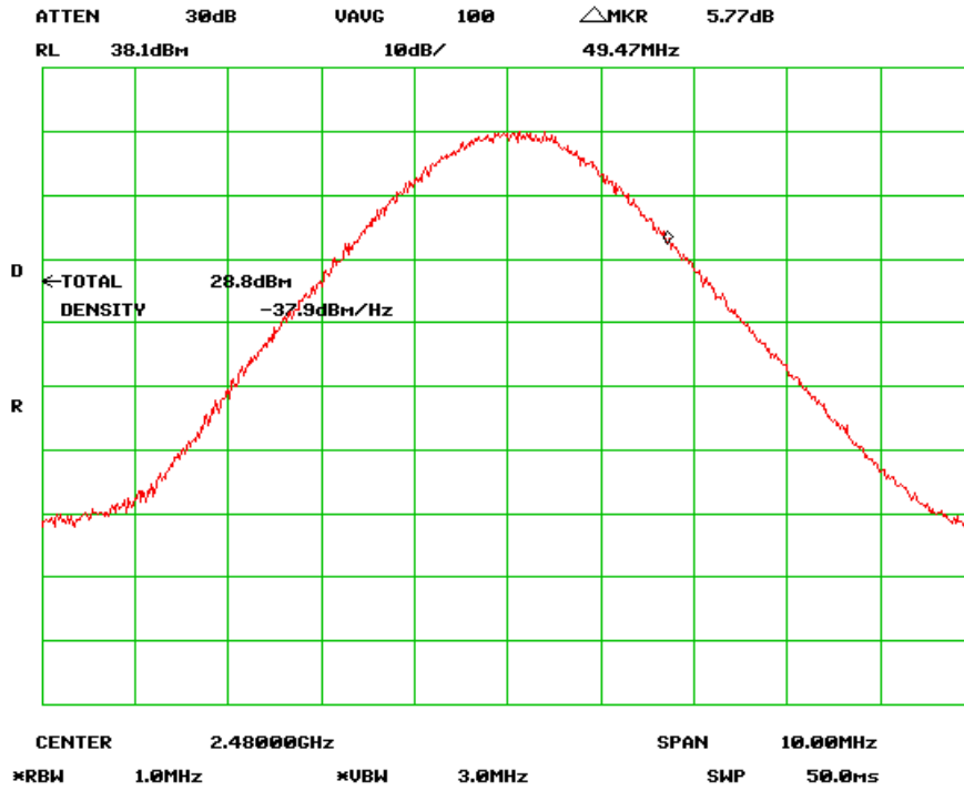
Output Power High Channel (Antenna Gain 9dBi)
