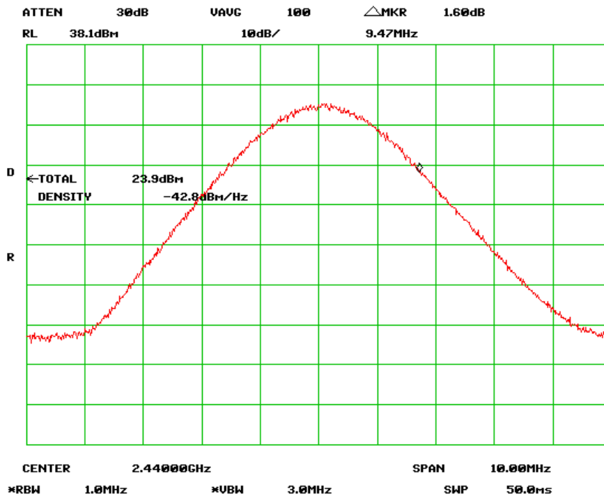
Output Power Middle Channel (Antenna Gain 24dB)
