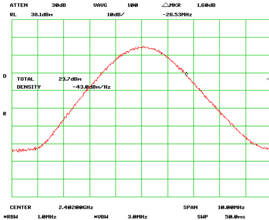
Output Power Low Channel (Antenna Gain 24dBi)
