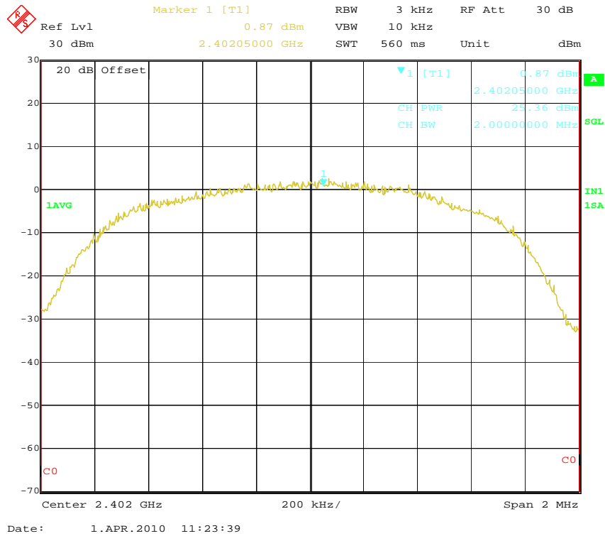
PSD Low Channel(9dBi) -1
