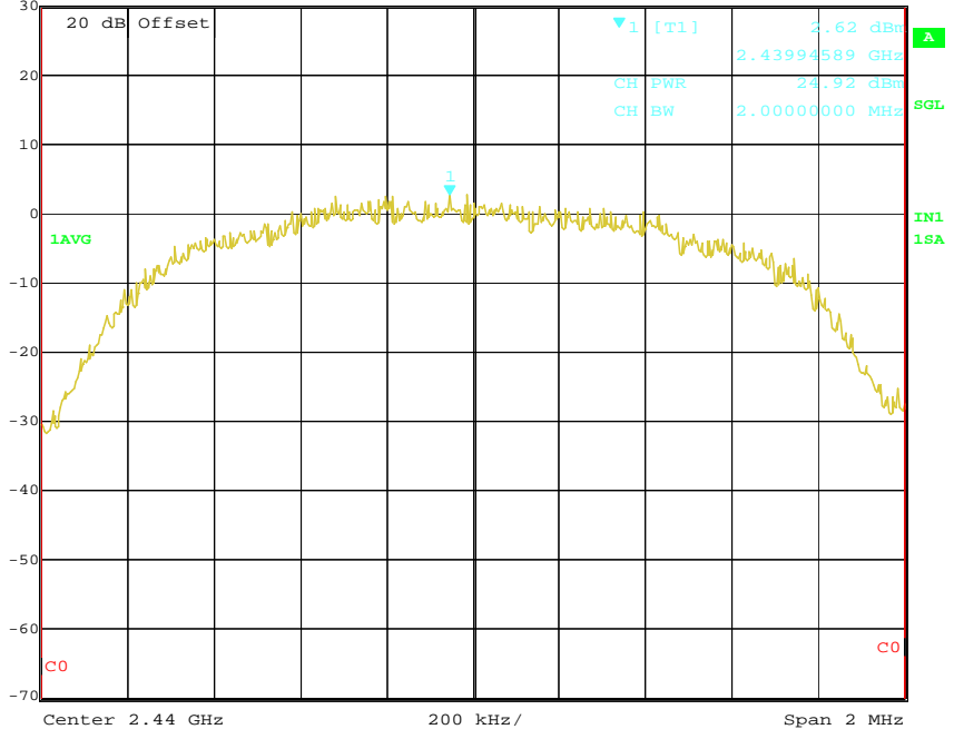
PSD Mid Channel(9dBi) -1
