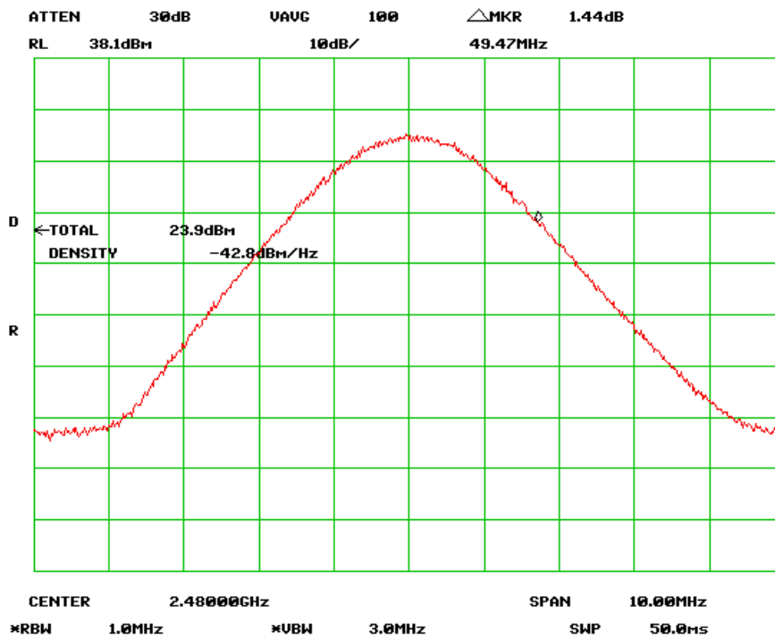
Output Power High Channel (Antenna Gain 24dB)
