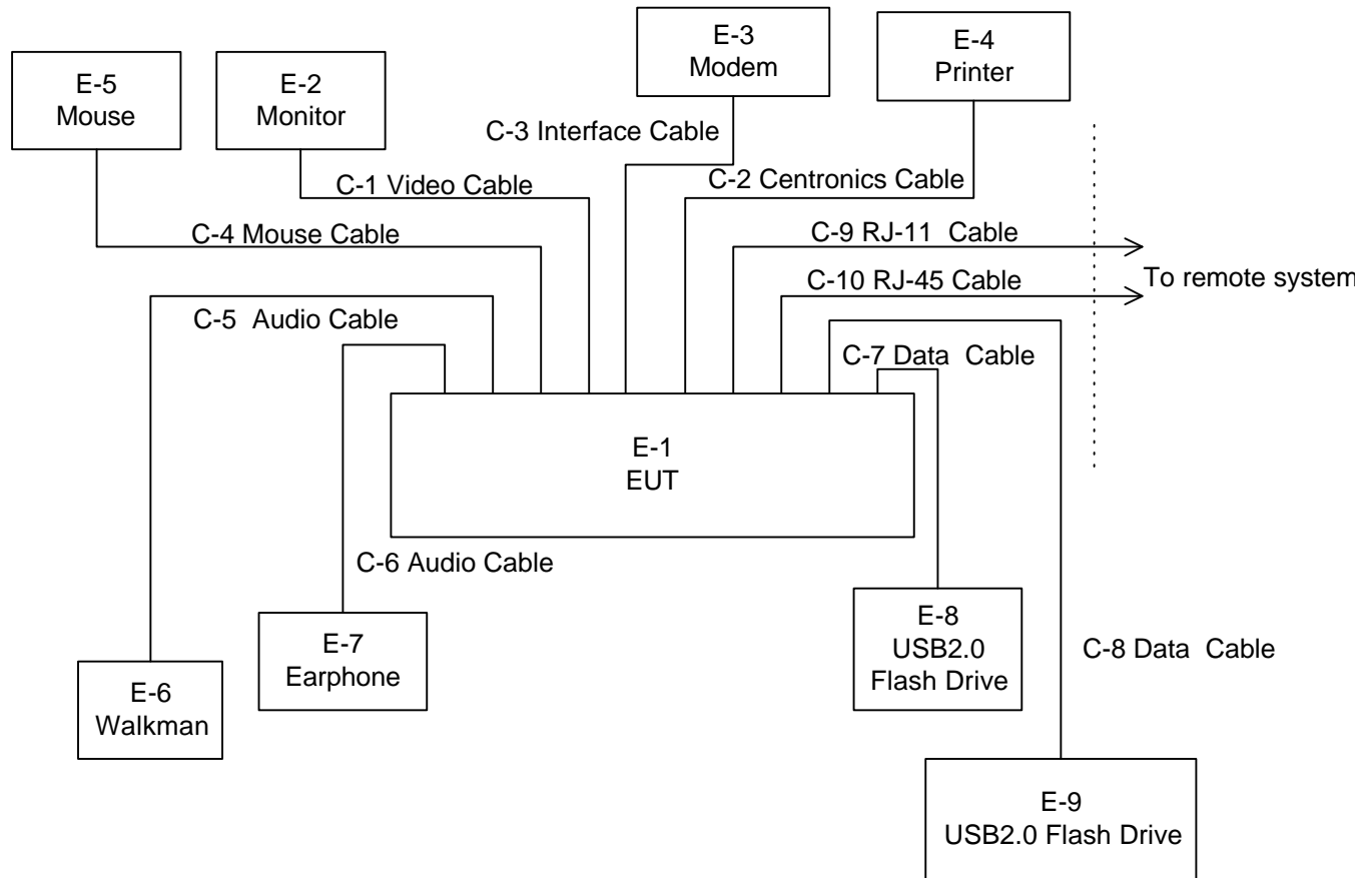
Diagram - 1 Block diagram showing the configuration of system tested
