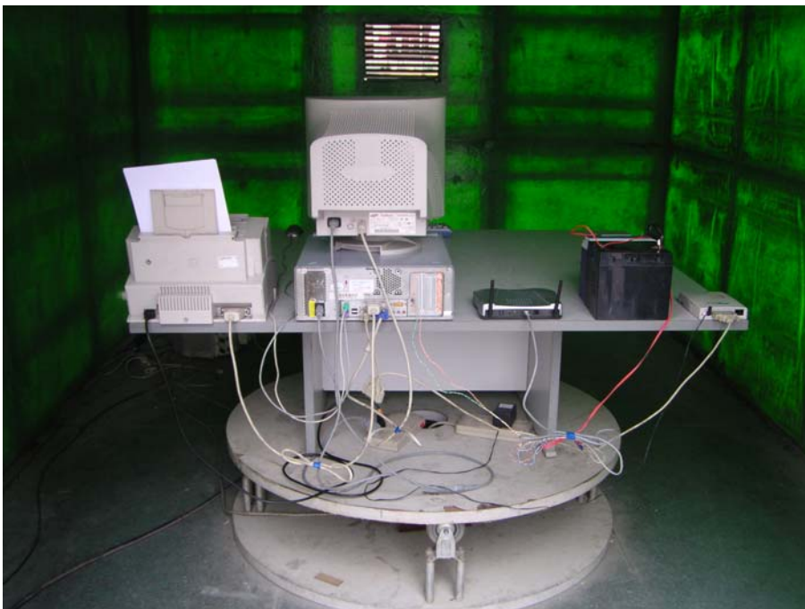
DC Power Antenna 9902-24-02-300/9902-24-02-110: Radiated Emission - Rear View
