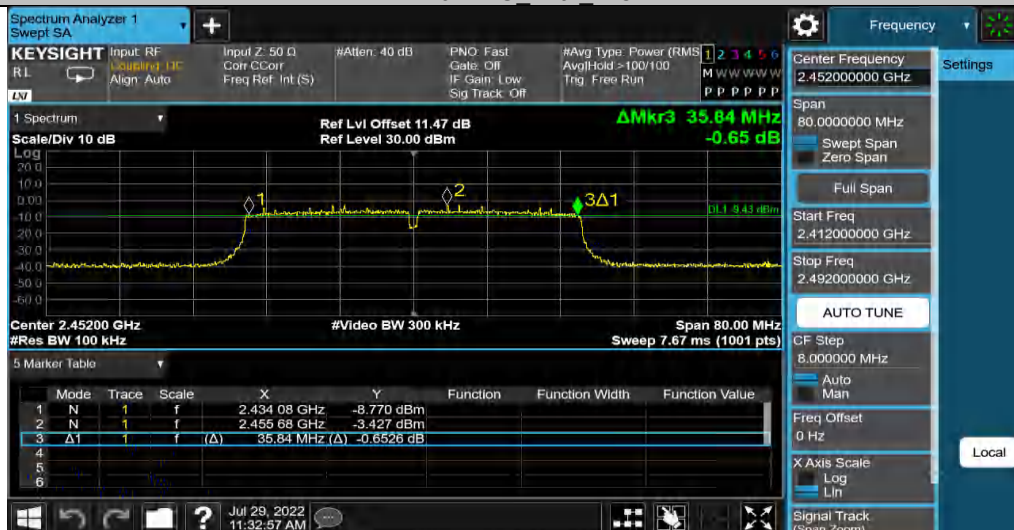
11N40MIMO Ant2 2452
