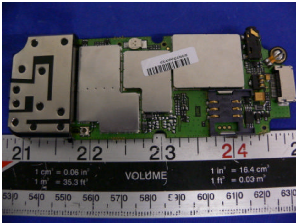
EUT Component with Shielding View
