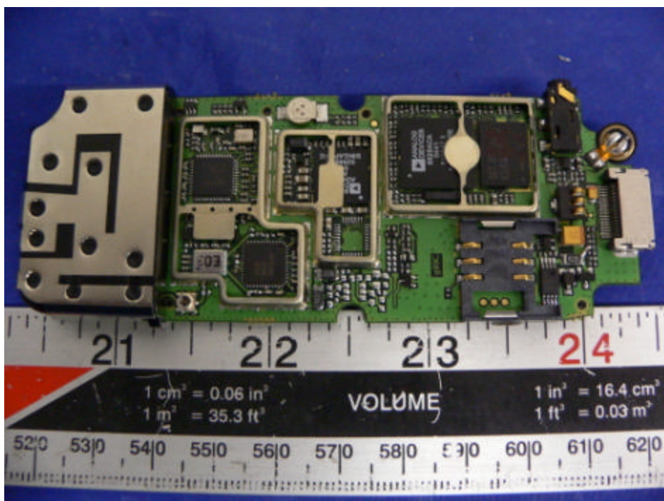
EUT Component without Shielding View
