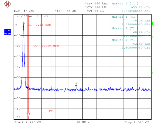
Bandedge CH78 (Upper)
