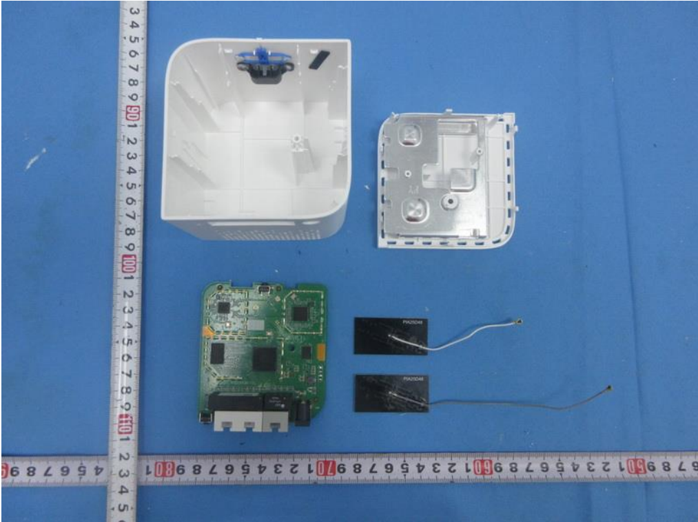
A PCB
