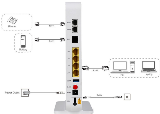
Figure 7-1 Entire Connection
