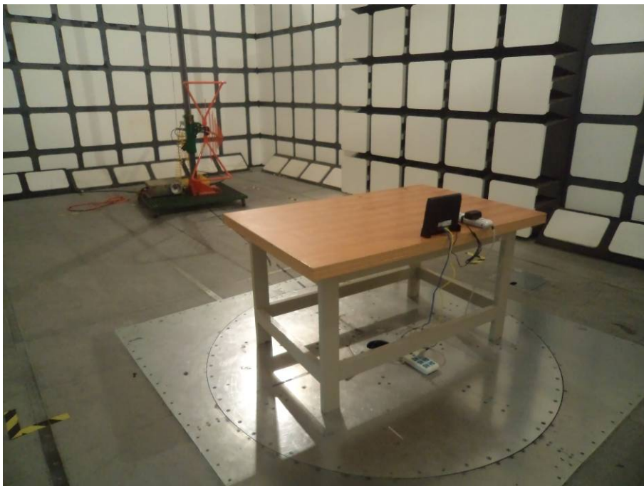
Radiated Emissions - Rear View (Adapter 1)
