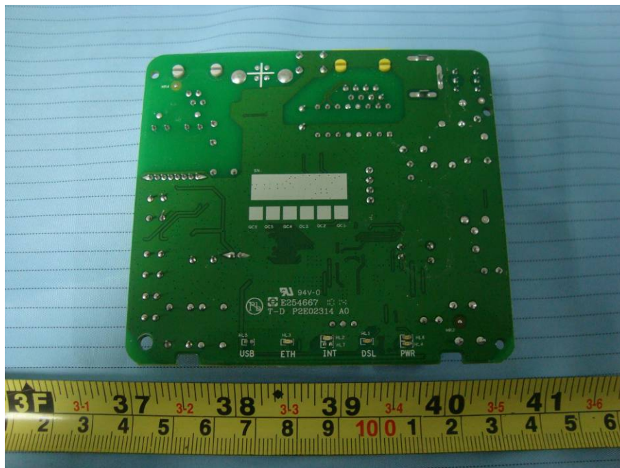
EUT – Main Board Bottom View (Model: ZXDSL 831 II)
