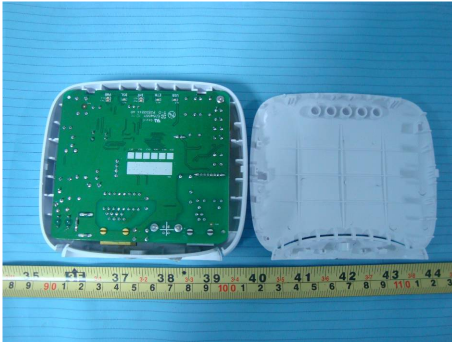
EUT – Cover off View (Model: ZXDSL 831A II)
