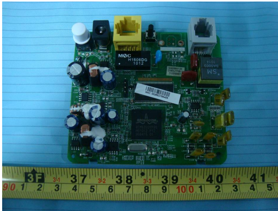
EUT – Main Board Top View (Model: ZXDSL 831 II)
