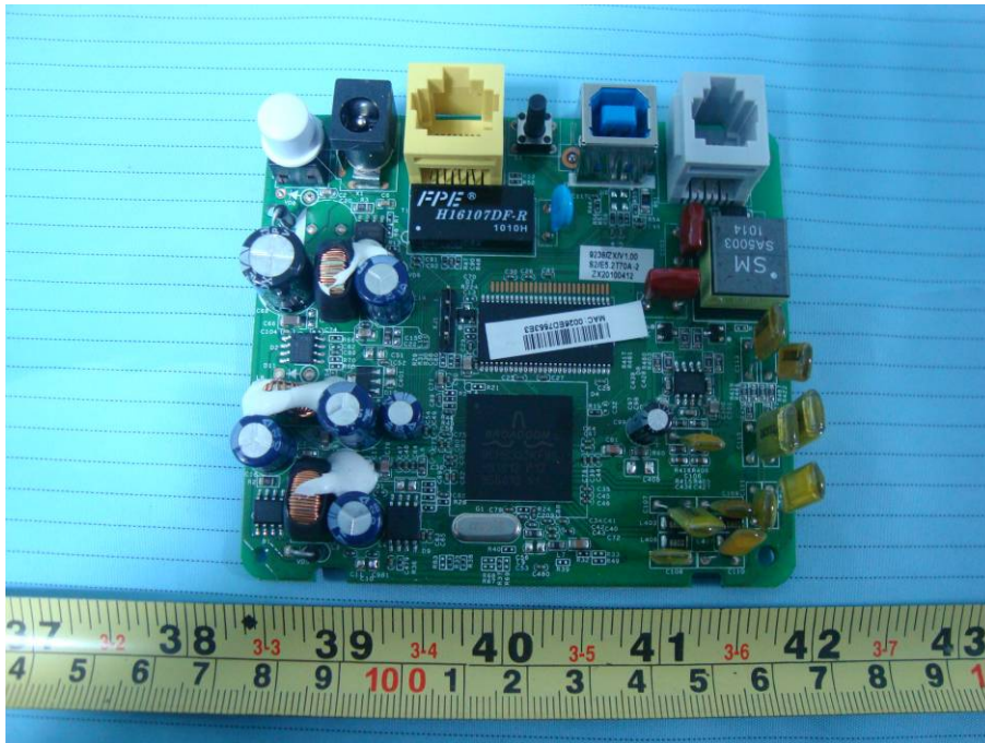
EUT – Main Board Top View (Model: ZXDSL 831A II)
