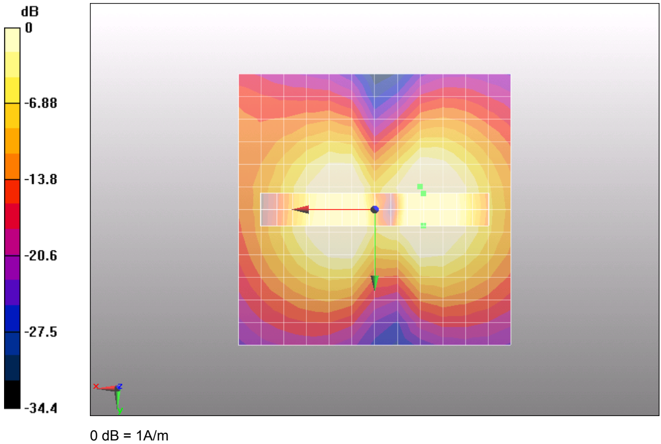
Figure 11 T-Coil GSM 850 X longitudinal
