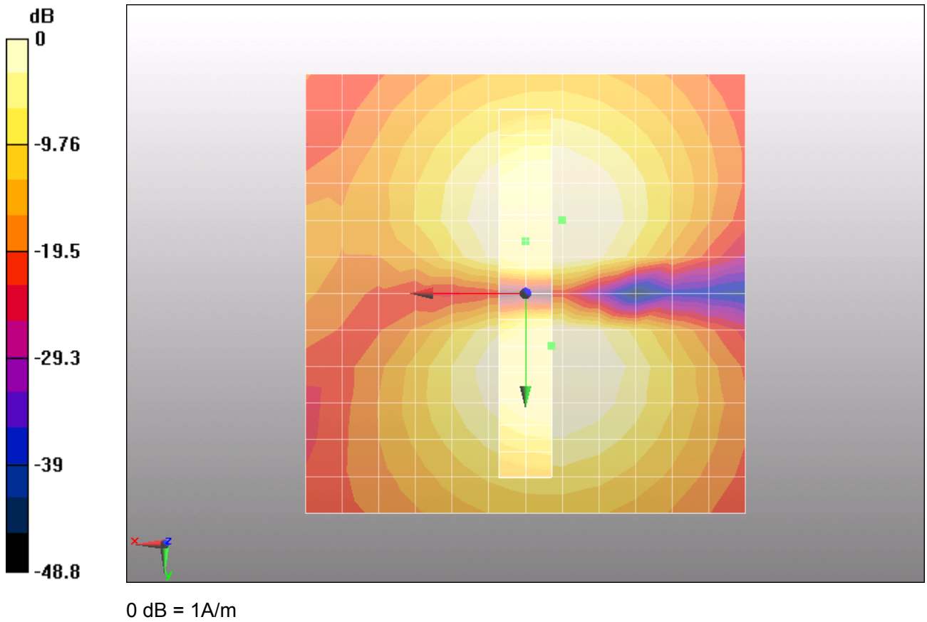
Figure 12 T-Coil GSM 850 Y transversal
