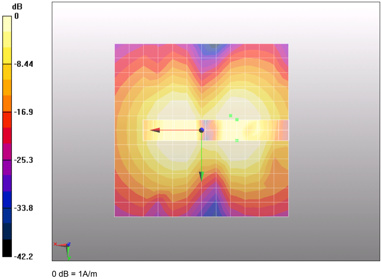
Figure 17 T-Coil WCDMA Band II X longitudinal
