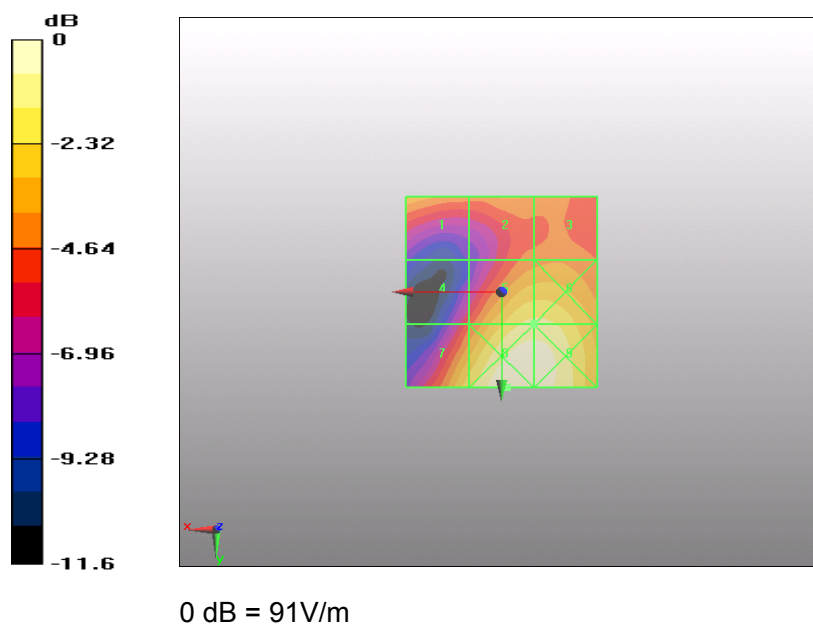
Figure 22 HAC RF E-Field GSM 1900 Channel 512
