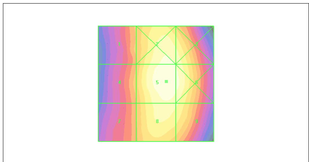
Figure 40 HAC RF E-Field WCDMA Band V Channel 4132
