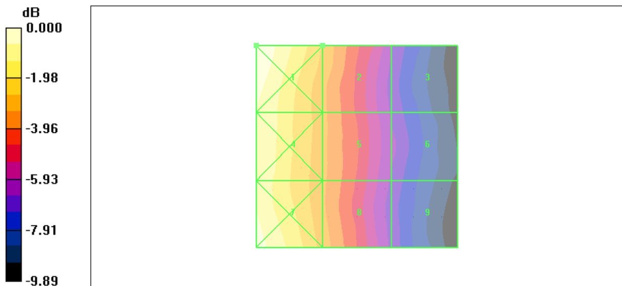
Figure 42 HAC RF H-Field WCDMA Band V Channel 4183
