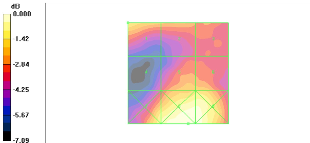
Figure 28 HAC RF E-Field WCDMA Band II Channel 9262
