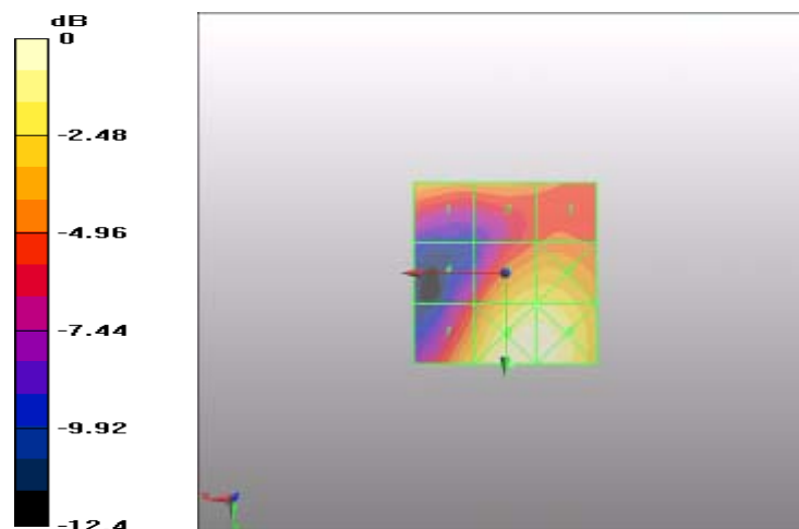
Figure 20 HAC RF E-Field GSM 1900 Channel 810
