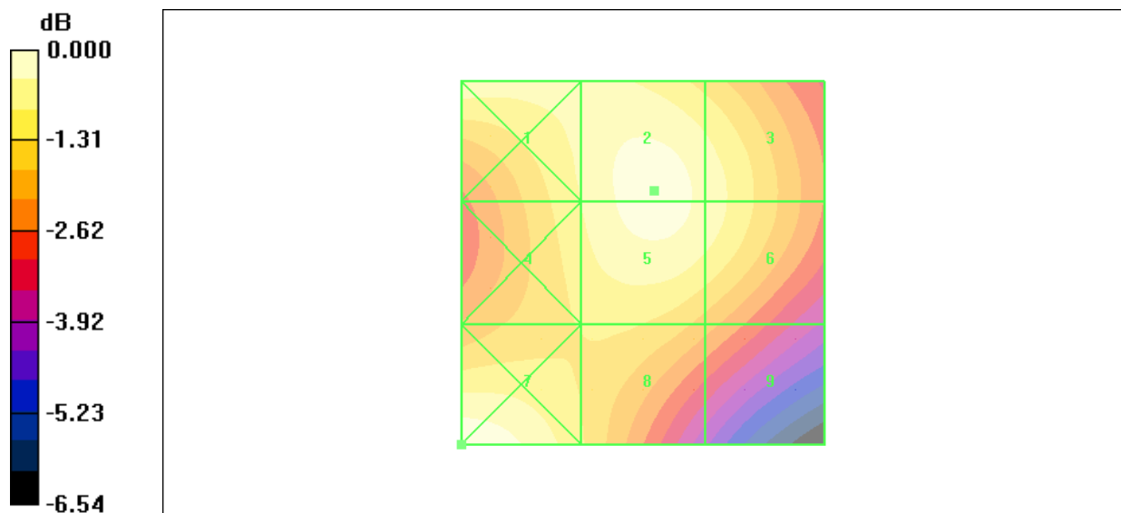
Figure 29 HAC RF H-Field WCDMA Band II Channel 9538
