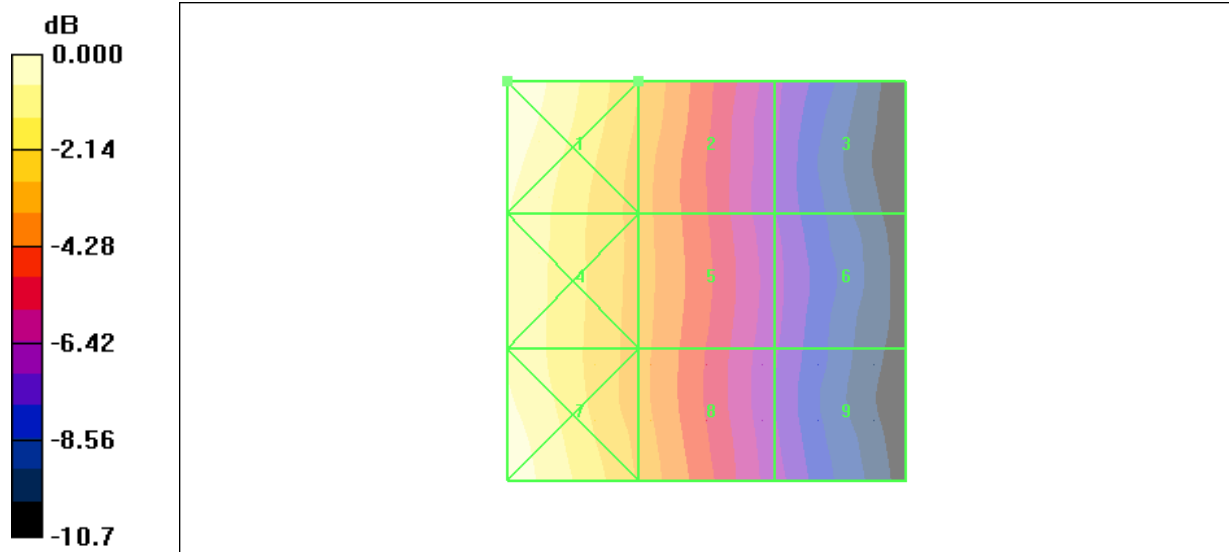
Figure 17 HAC RF H-Field GSM 850Channel 251
