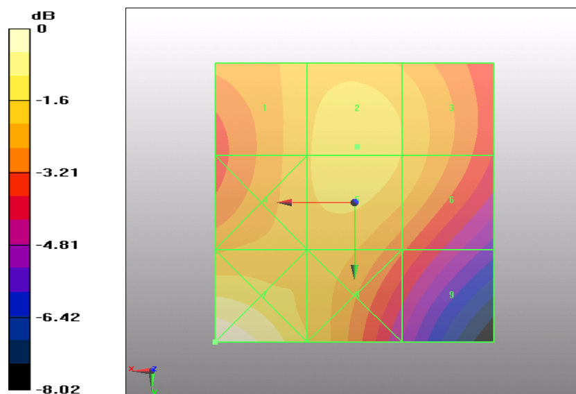
Figure 35 HAC RF H-Field WCDMA Band IV Channel 1513
