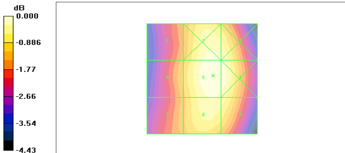
Figure 14 HAC RF E-Field GSM 850 Channel 251
