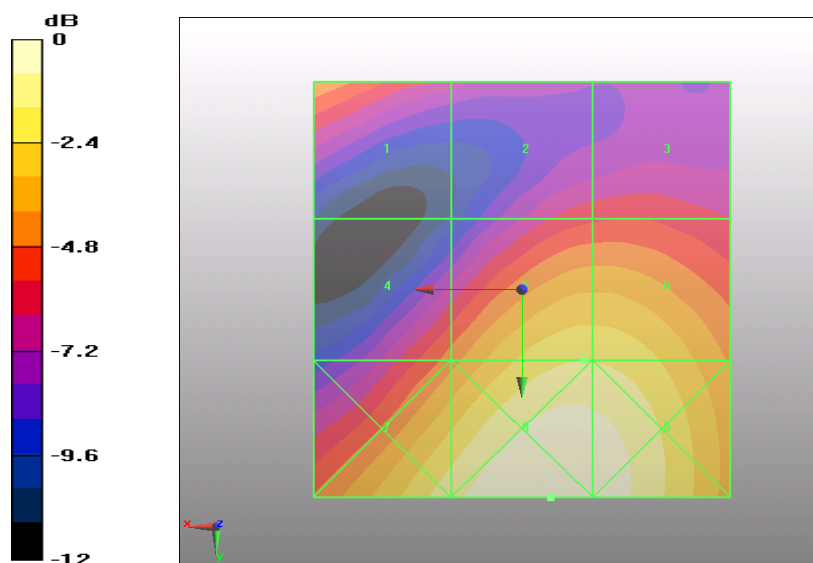
Figure 34 HAC RF E-Field WCDMA Band IV Channel 1312
