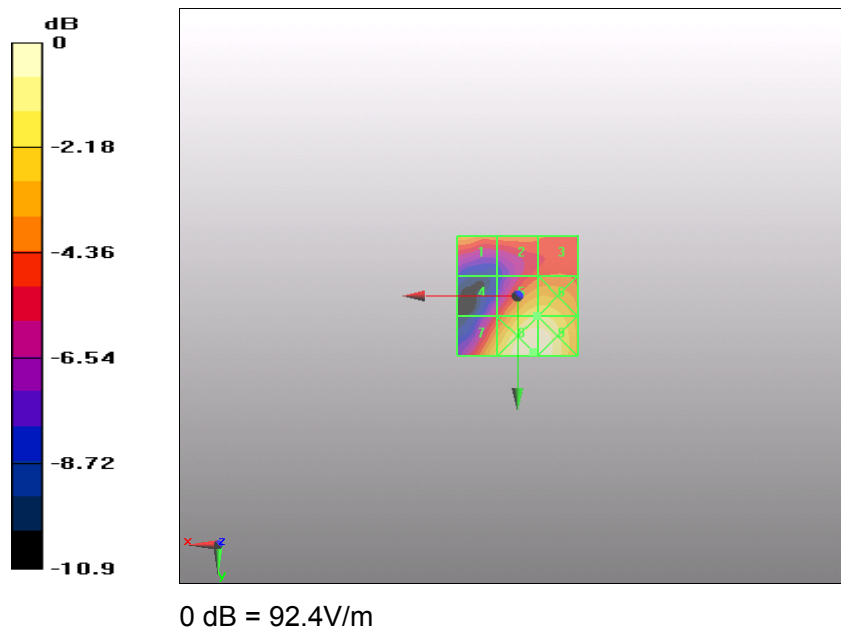
Figure 21 HAC RF E-Field GSM 1900 Channel 661
