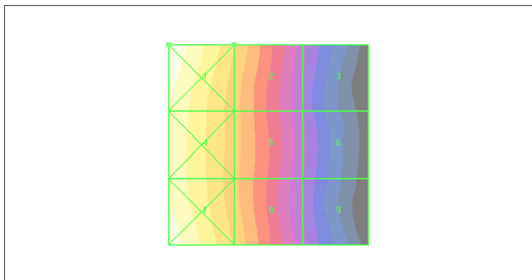
Figure 19 HAC RF H-Field GSM 850 Channel 128
