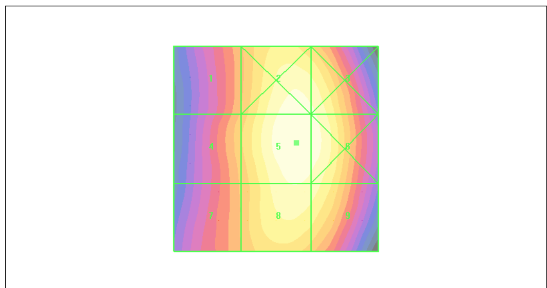
Figure 38 HAC RF E-Field WCDMA Band V Channel 4233
