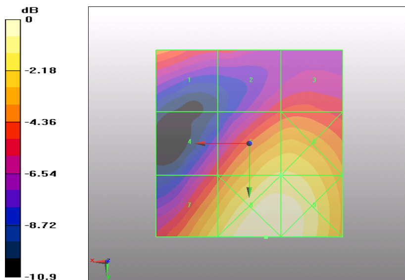
Figure 33 HAC RF E-Field WCDMA Band IV Channel 1413
