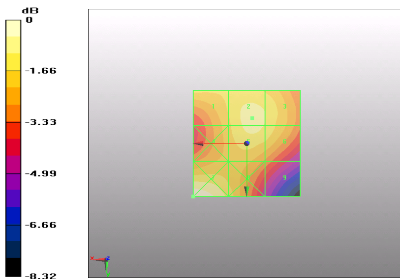
Figure 23 HAC RF H-Field GSM 1900 Channel 810
