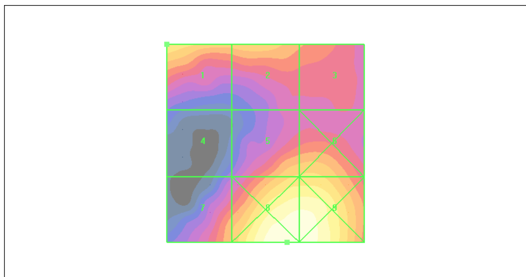
Figure 26 HAC RF E-Field WCDMA Band II Channel 9538
