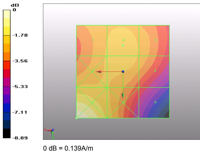
Figure 36 HAC RF H-Field WCDMA Band IV Channel 1413
