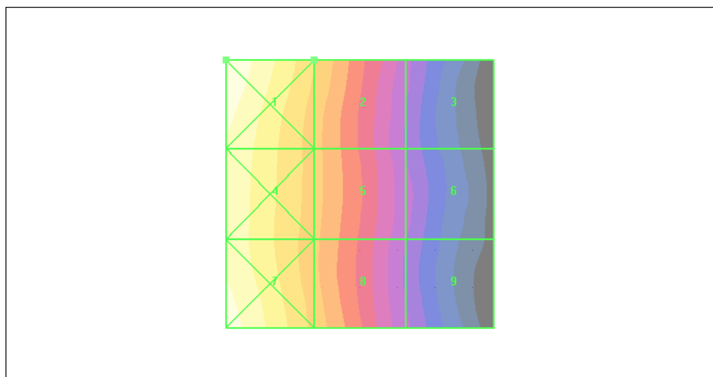
Figure 41 HAC RF H-Field WCDMA Band V Channel 4233
