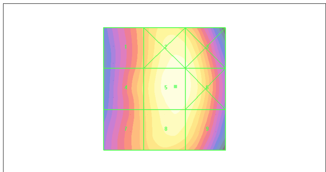
Figure 15 HAC RF E-Field GSM 850 Channel 190
