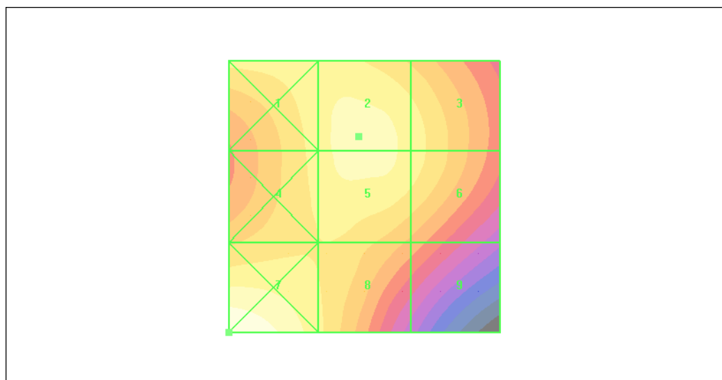
Figure 31 HAC RF H-Field WCDMA Band II Channel 9262
