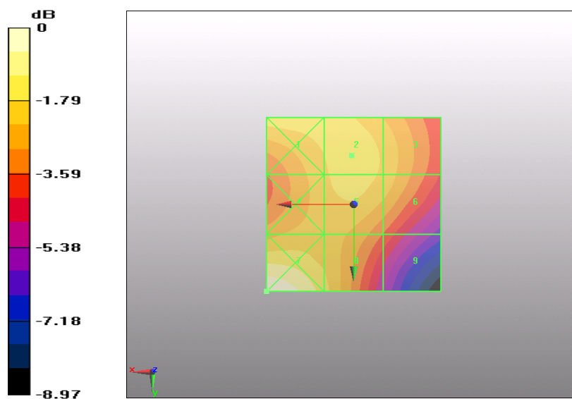
Figure 25 HAC RF H-Field GSM 1900 Channel 512
