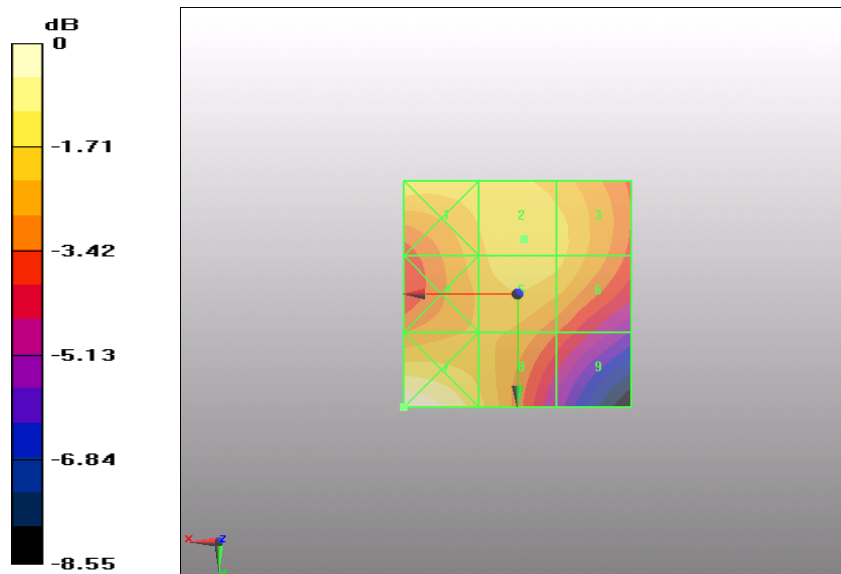
Figure 24 HAC RF H-Field GSM 1900 Channel 661
