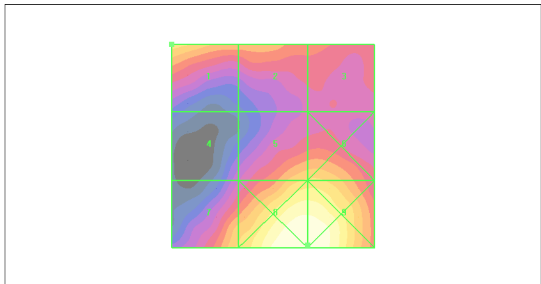
Figure 27 HAC RF E-Field WCDMA Band II Channel 9400
