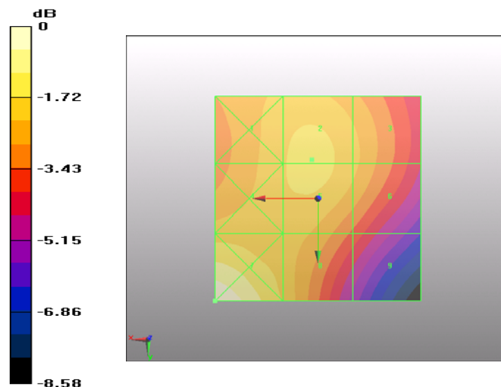
Figure 37 HAC RF H-Field WCDMA Band IV Channel 1312
