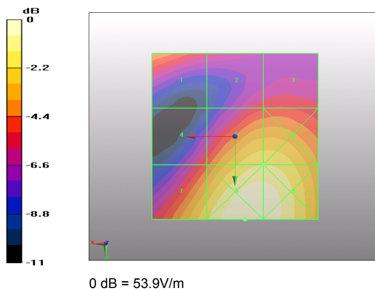
Figure 32 HAC RF E-Field WCDMA Band IV Channel 1513
