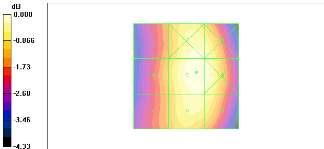
Figure 16 HAC RF E-Field GSM 850 Channel 128
