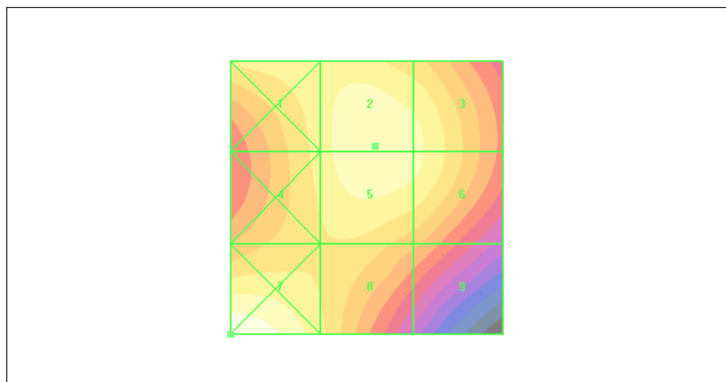
Figure 30 HAC RF H-Field WCDMA Band II Channel 9400
