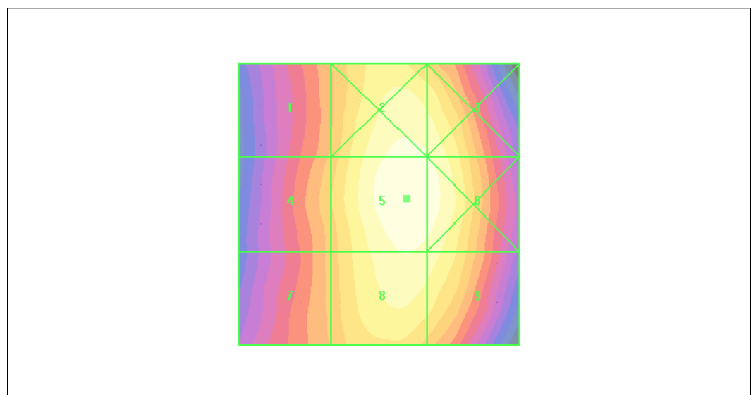
Figure 39 HAC RF E-Field WCDMA Band V Channel 4183
