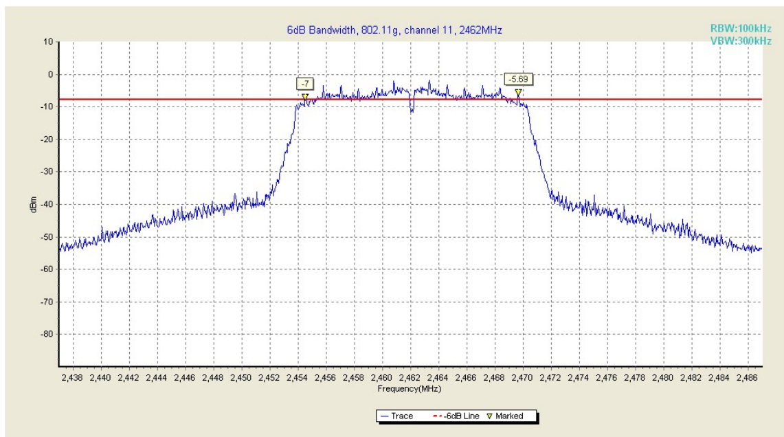
Fig. 15 Occupied 6dB Bandwidth (802.11g, Ch 11)
