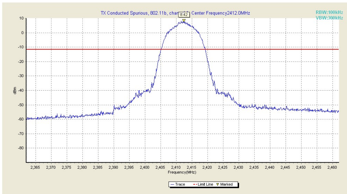
Fig. 25 Conducted Spurious Emission (802.11b, Ch1, Center Frequency)
