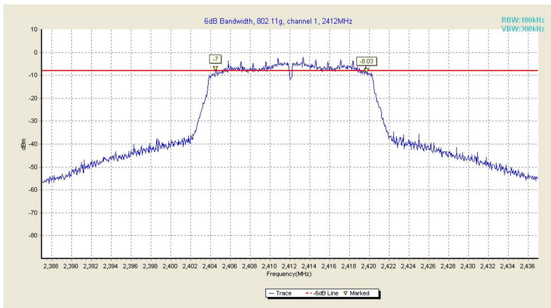
Fig. 13 Occupied 6dB Bandwidth (802.11g, Ch 1)
