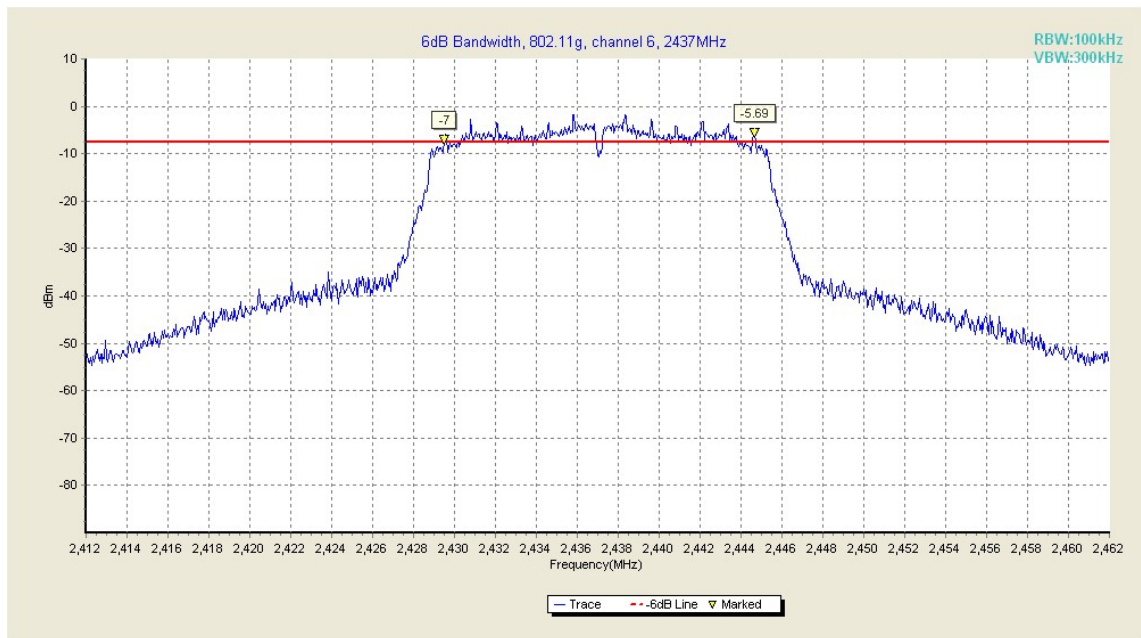
Fig. 14 Occupied 6dB Bandwidth (802.11g, Ch 6)
