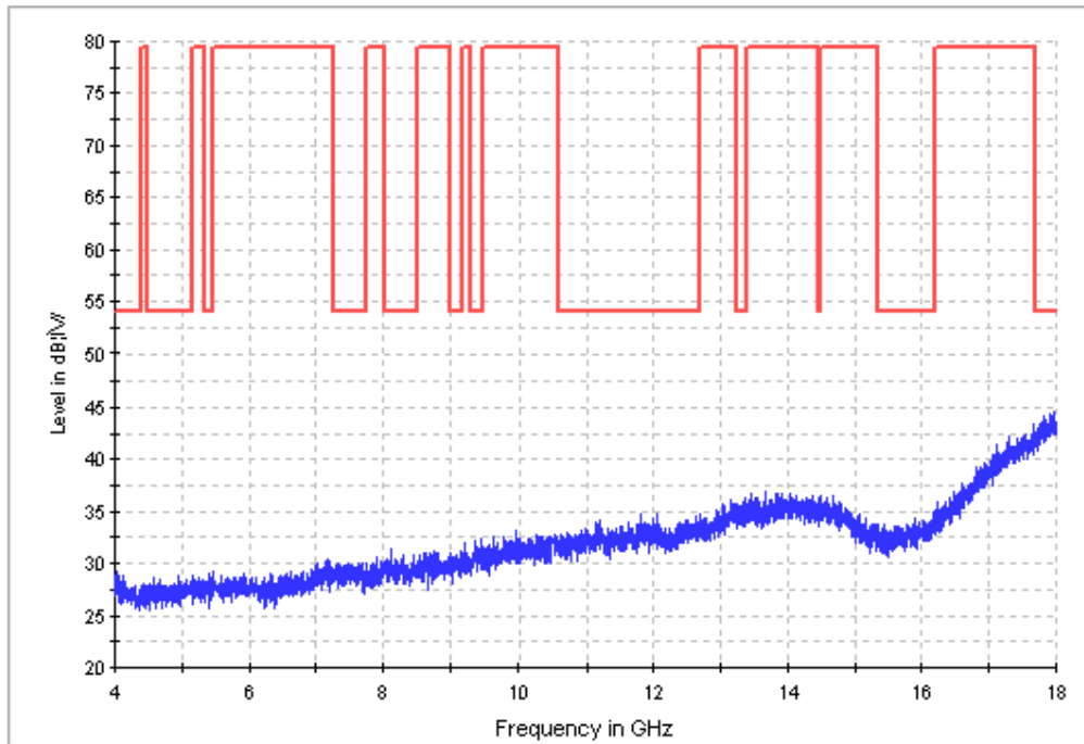
Fig. 64 Radiated Spurious Emission (802.11g, Ch11, 4 GHz-18 GHz)
