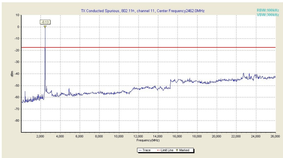
Fig. 42 Conducted Spurious Emission (802.11n-20MHz, Ch11, 30 MHz-26 GHz)
