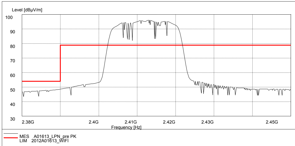
Fig. 65 Radiated Spurious Emission (Power): 802.11n-20MHz, ch1, 2.38 GHz - 2.45GHz
