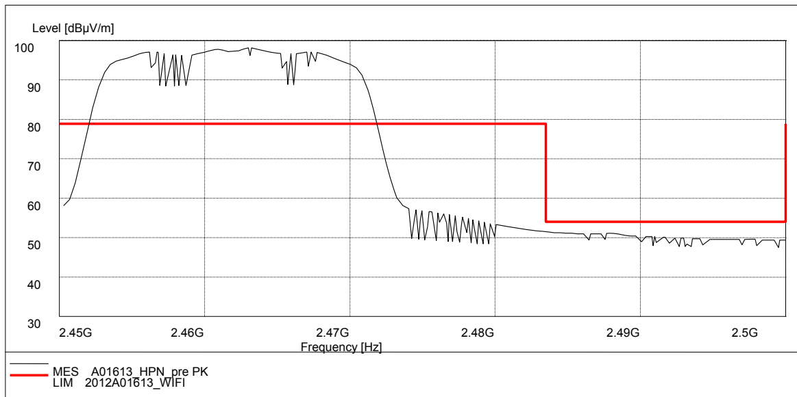
Fig. 72 Radiated Spurious Emission (Power): 802.11n-20MHz, ch11, 2.45 GHz - 2.50GHz
