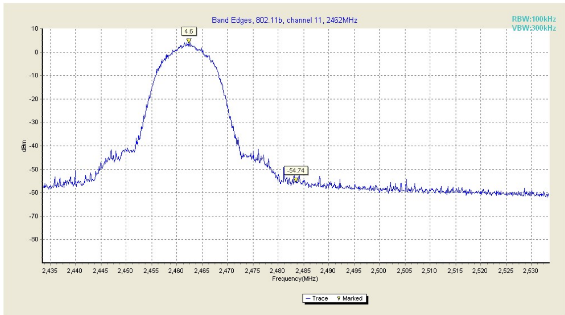
Fig. 20 Band Edges (802.11b, Ch 11)
