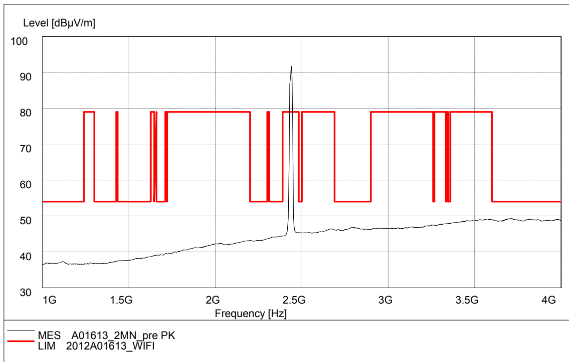
Fig. 70 Radiated Spurious Emission (802.11n-20MHz, Ch6, 1 GHz-4 GHz)
