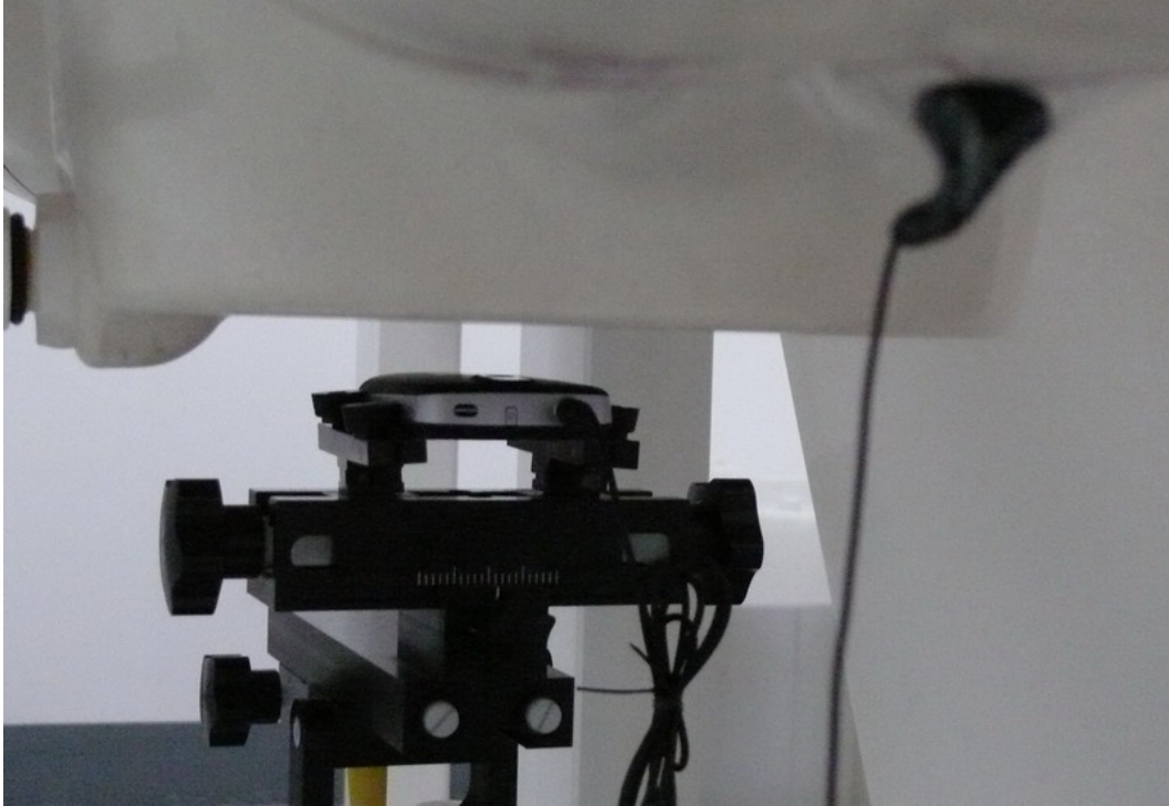
Picture 15: Body with earphone, The EUT display towards ground, the distance from handset to the bottom of the Phantom is 15mm
