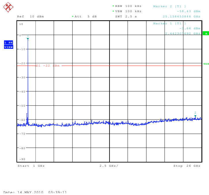
Fig. 27 Conducted spurious emission: \pi/4 DQPSK, Channel 39, 1GHz – 26GHz
