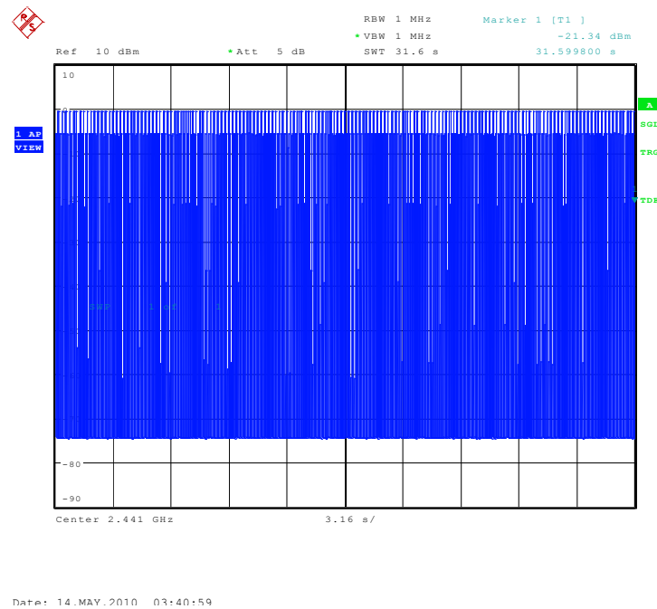
Fig. 80 Number of Transmissions Measurement:Channel 39,Packet 2-DH1
