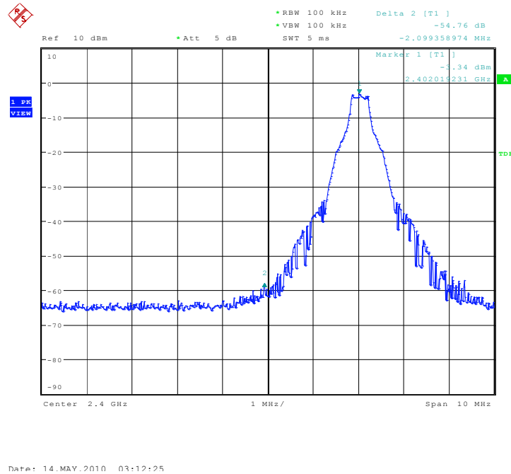
Fig. 1 Frequency Band Edges: GFSK, Channel 0, Hopping Off
