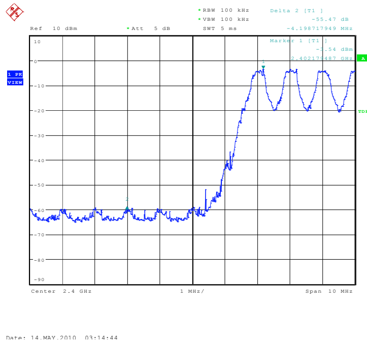
Fig. 2 Frequency Band Edges: GFSK, Channel 0, Hopping On
