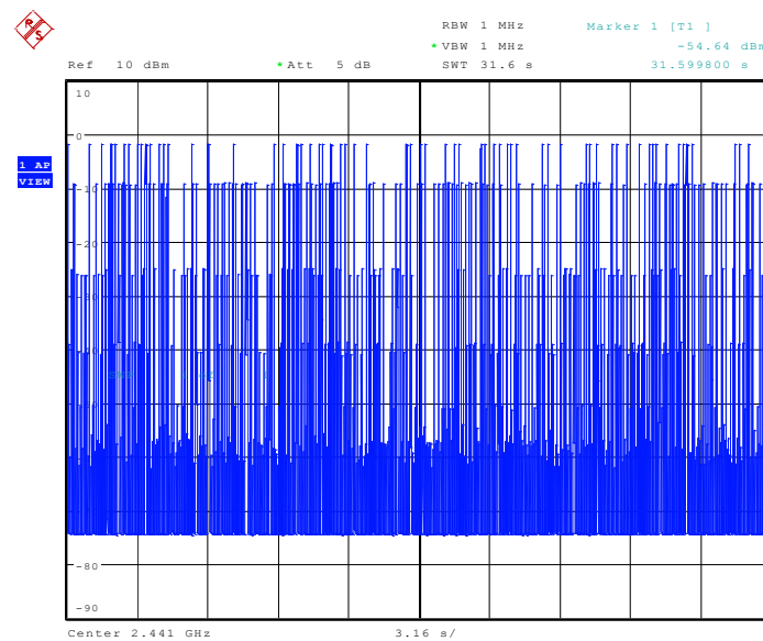
Fig. 77 Time of occupancy (Dwell Time): Channel 39, Packet DH5
