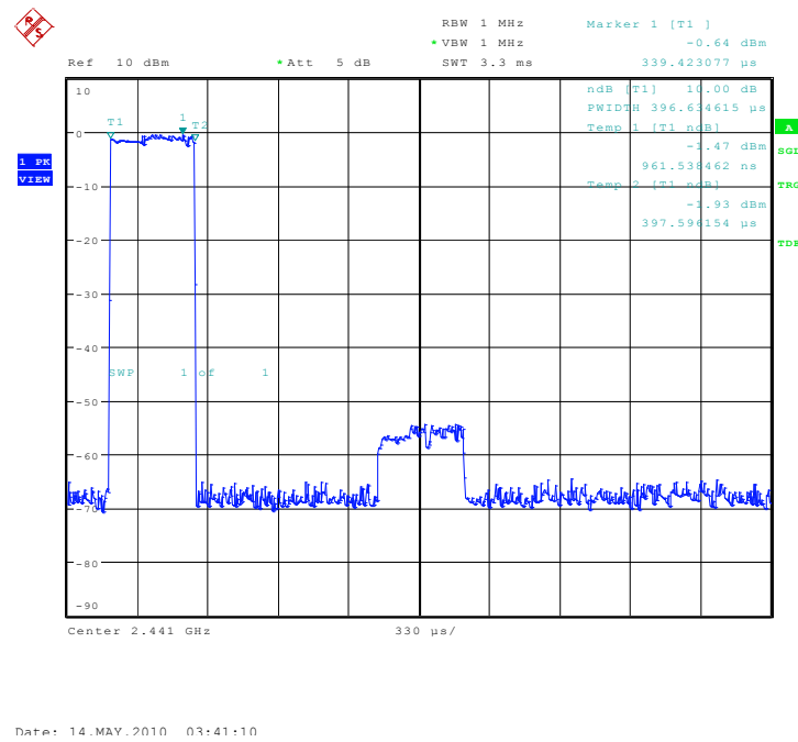
Fig. 79 Time of occupancy (Dwell Time): Channel 39, Packet 2-DH1
