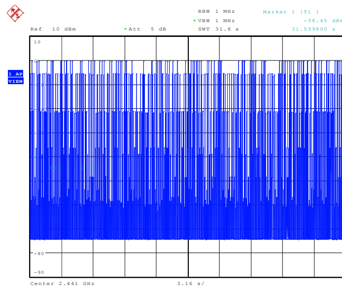
Fig. 81 Time of occupancy (Dwell Time): Channel 39, Packet 2-DH3
