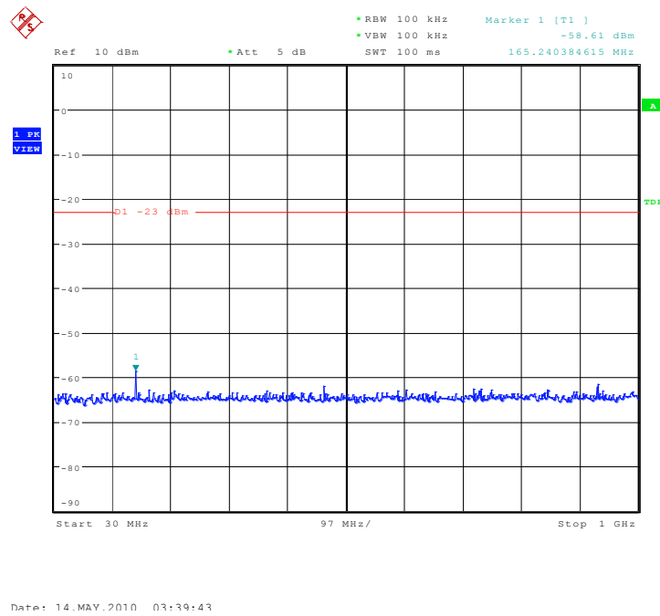
Fig. 29 Conducted spurious emission: \pi/4 DQPSK, Channel 78, 30MHz - 1GHz
