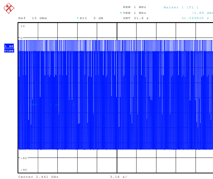
Fig. 73 Time of occupancy (Dwell Time): Channel 39, Packet DH1
