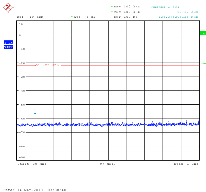
Fig. 26 Conducted spurious emission: \pi/4 DQPSK, Channel 39, 30MHz - 1GHz
