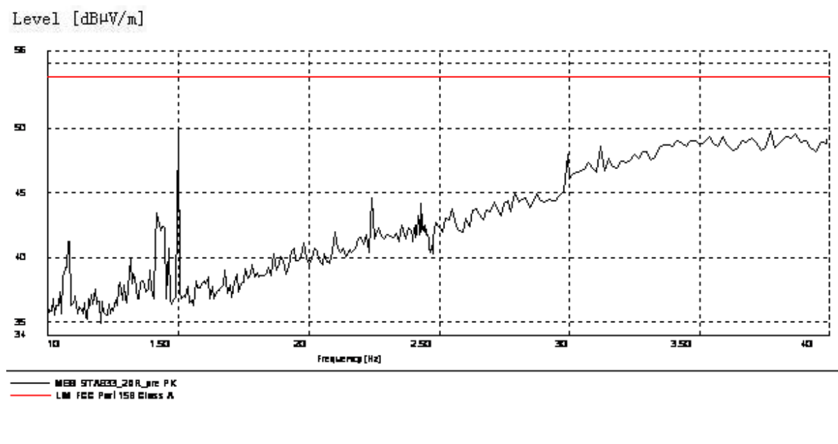
Figure A.2 Radiated Emission from 1GHz to 4GHz
