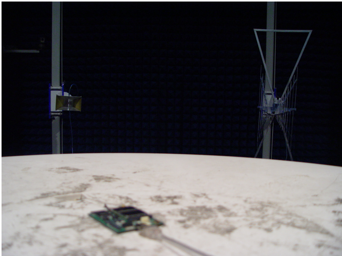
Radiated Spurious Emissions Test setup2
