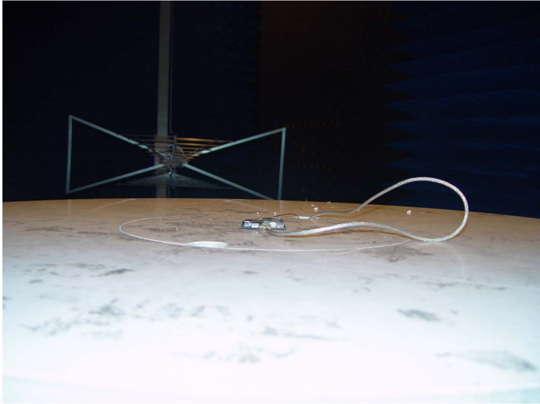
Radiated Spurious Emissions Test setup1
