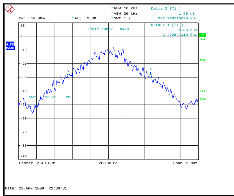
Fig. 30 20dB Bandwidth: Channel 78
