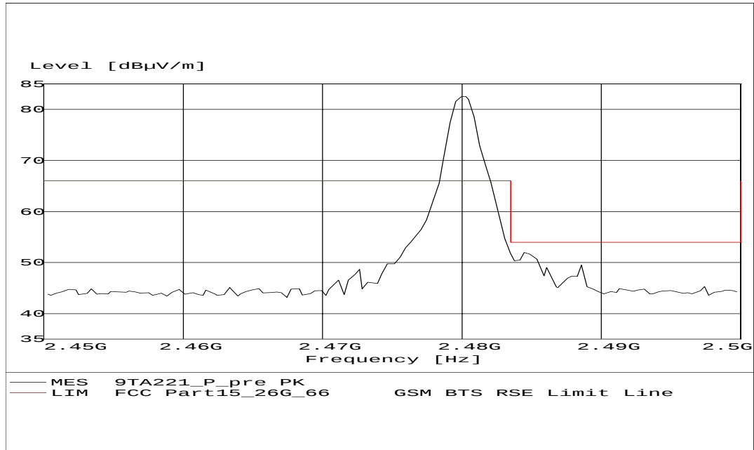
Fig. 23 Radiated emission (Power): channel 78, 2.45GHz ~ 2.5GHz
