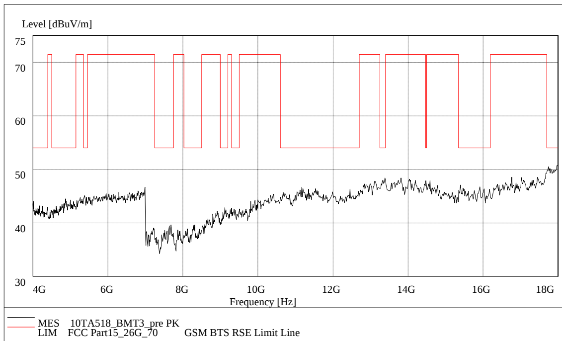
Fig. 41 Radiated Spurious Emission (802.11b, Ch6, 4 GHz-18 GHz)
