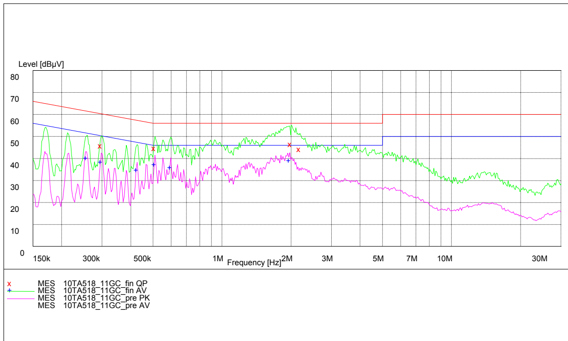
Fig. 57 AC Powerline Conducted Emission - 802.11g mode
