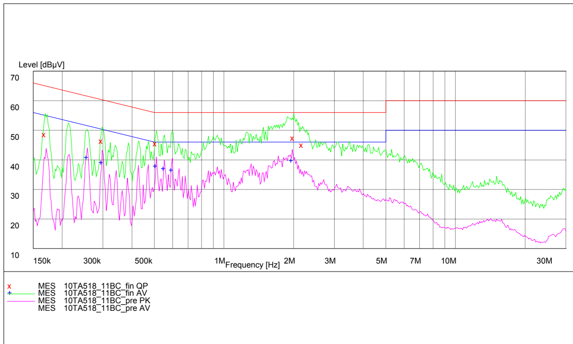
Fig. 56 AC Powerline Conducted Emission - 802.11b mode
