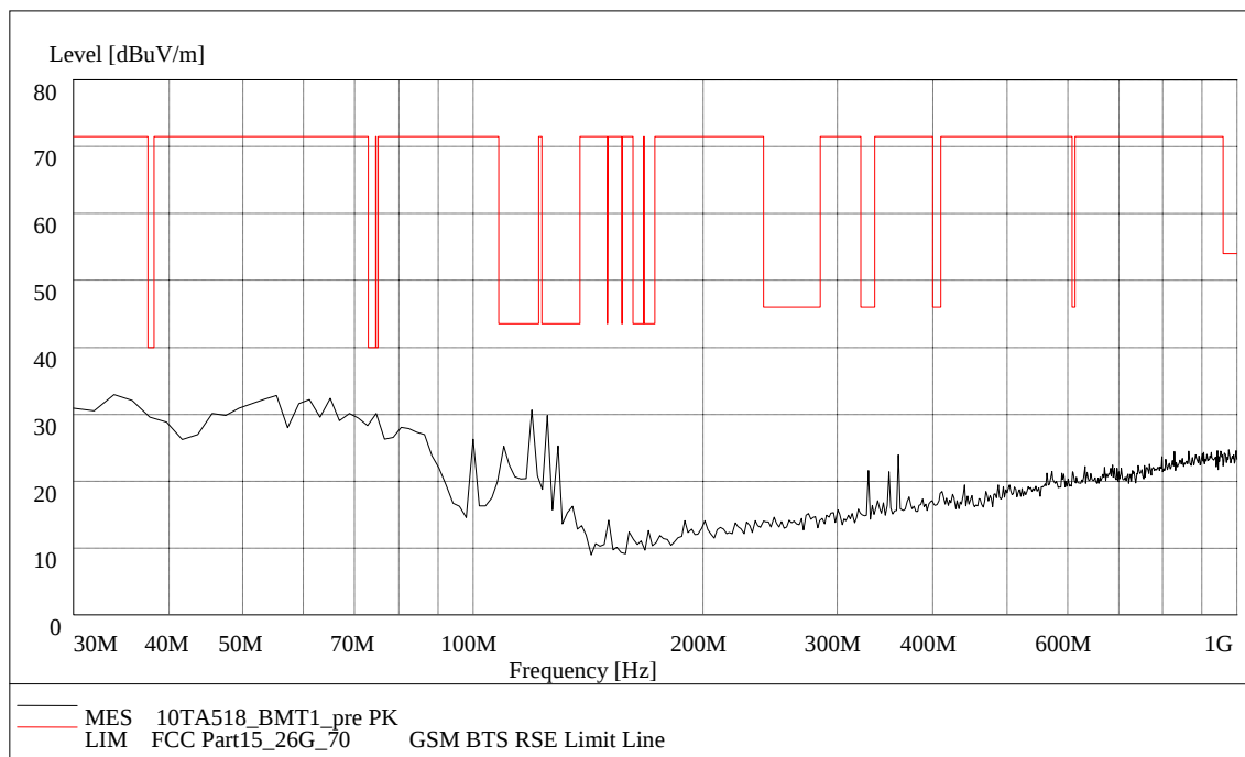
Fig. 39 Radiated Spurious Emission (802.11b, Ch6, 30 MHz-1 GHz)
