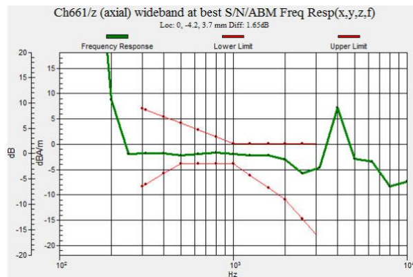
Fig 7.2 GSM1900 Ch661
