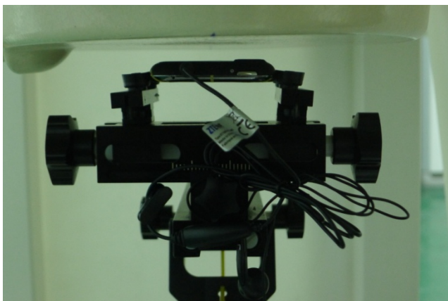
Back of the DUT with Phantom 1 cm Gap (w/ Headset)
