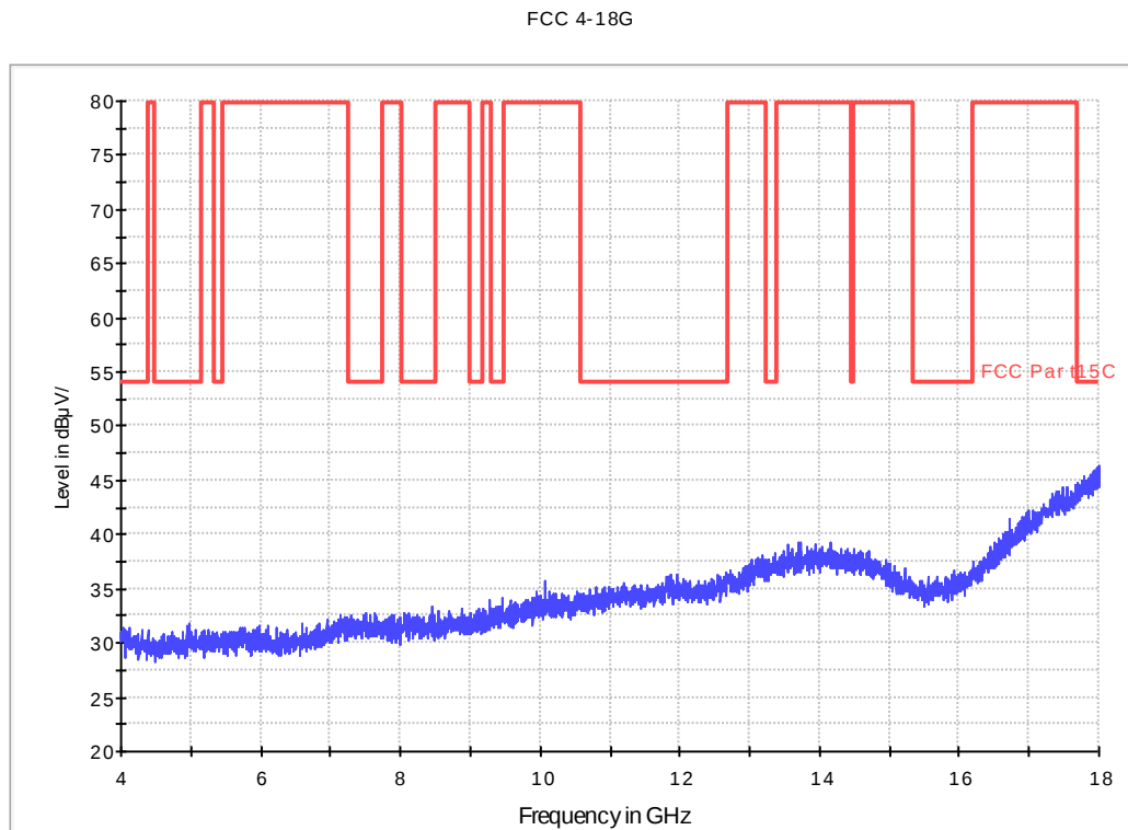
Fig. 79 Radiated Spurious Emission (802.11g, Ch1, 4 GHz-18 GHz)
