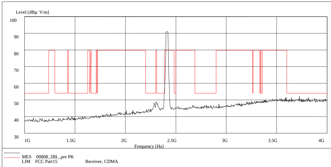
Fig. 67 Radiated Spurious Emission (802.11b, Ch1, 1 GHz-4 GHz)
