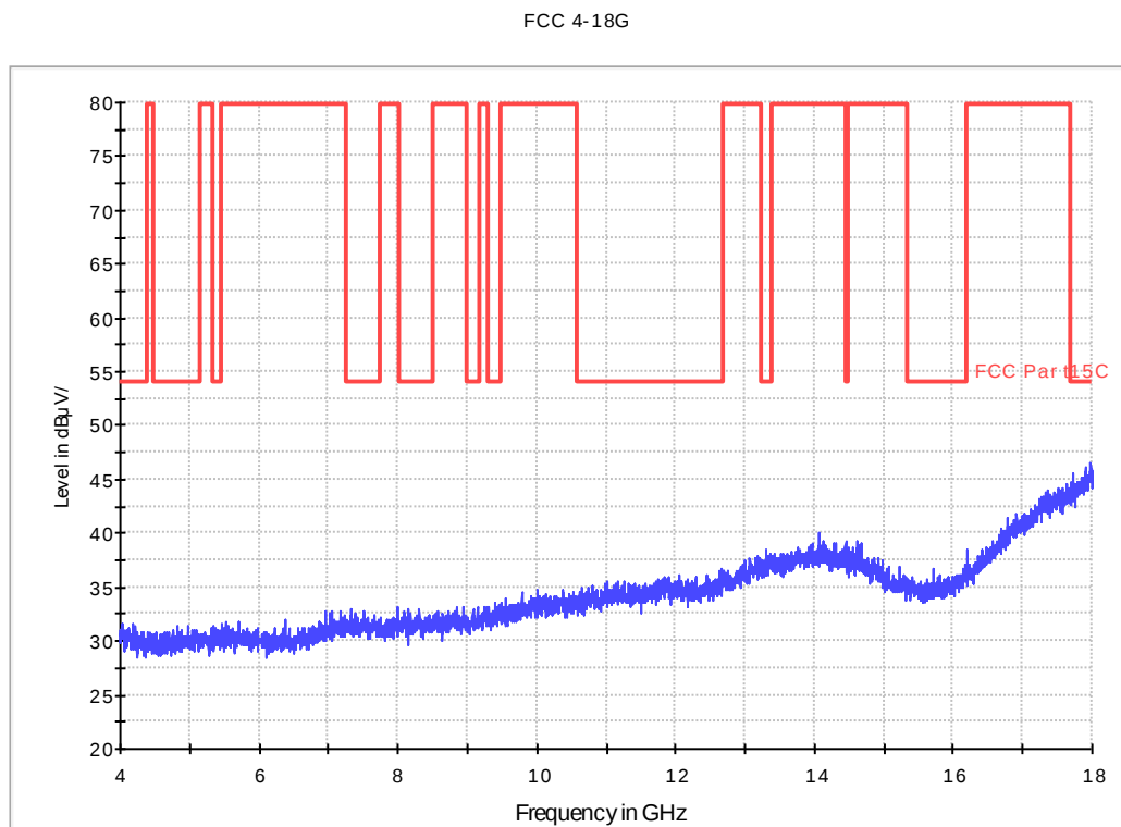
Fig. 86 Radiated Spurious Emission (802.11g, Ch11, 4 GHz-18 GHz)
