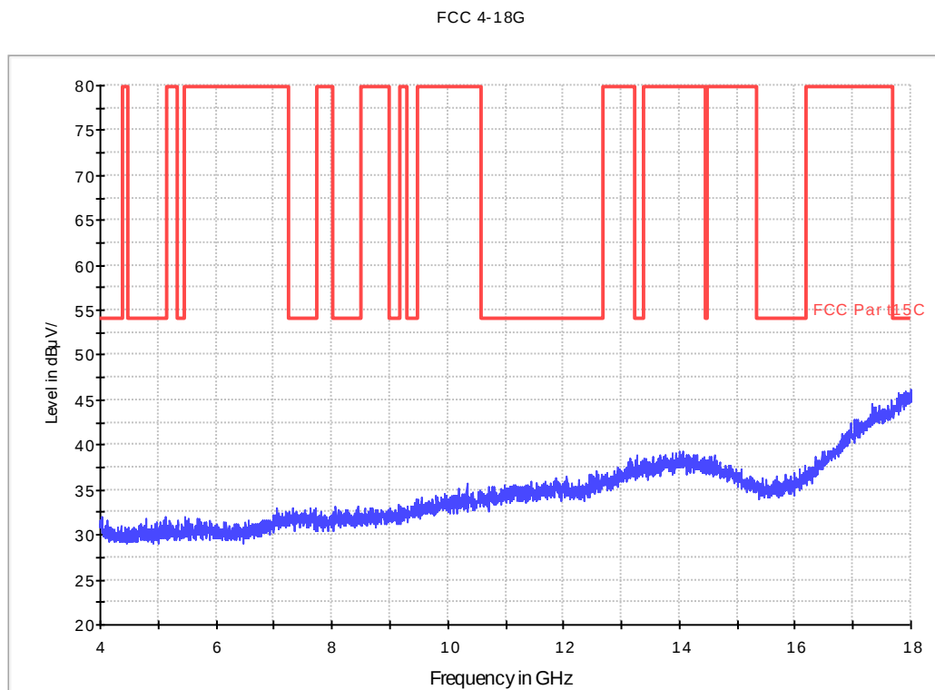
Fig. 68 Radiated Spurious Emission (802.11b, Ch1, 4 GHz-18 GHz)
