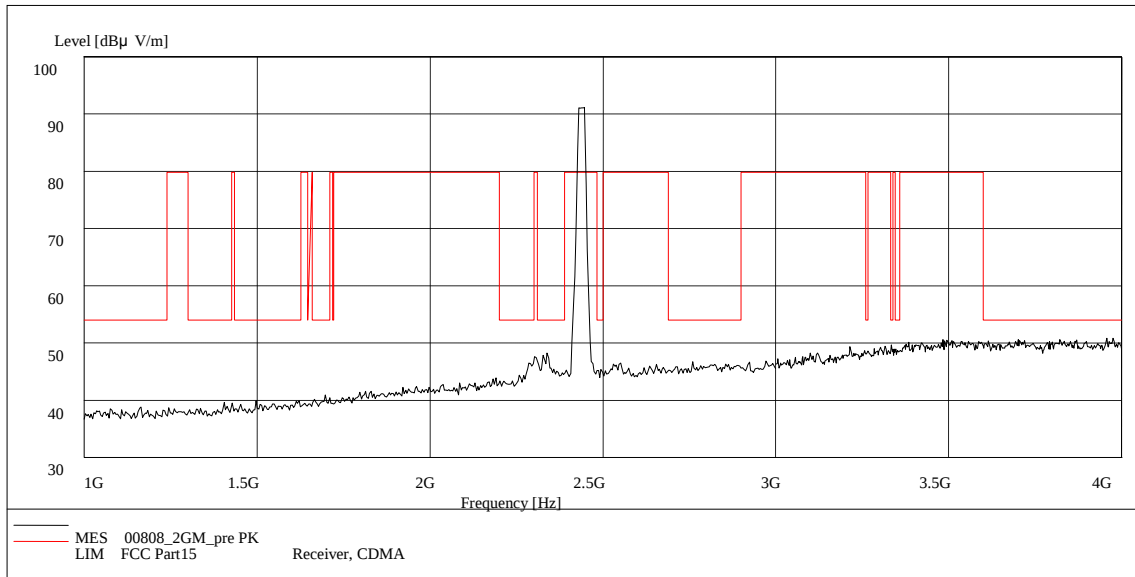
Fig. 81 Radiated Spurious Emission (802.11g, Ch6, 1 GHz-4 GHz)
