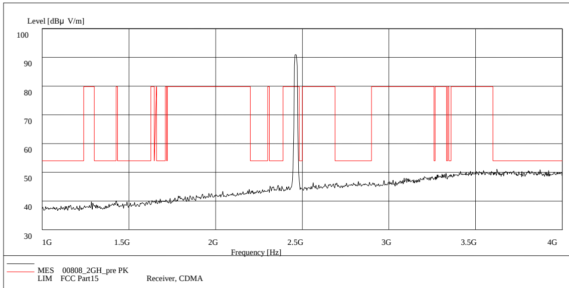
Fig. 85 Radiated Spurious Emission (802.11g, Ch11, 1 GHz-4 GHz)
