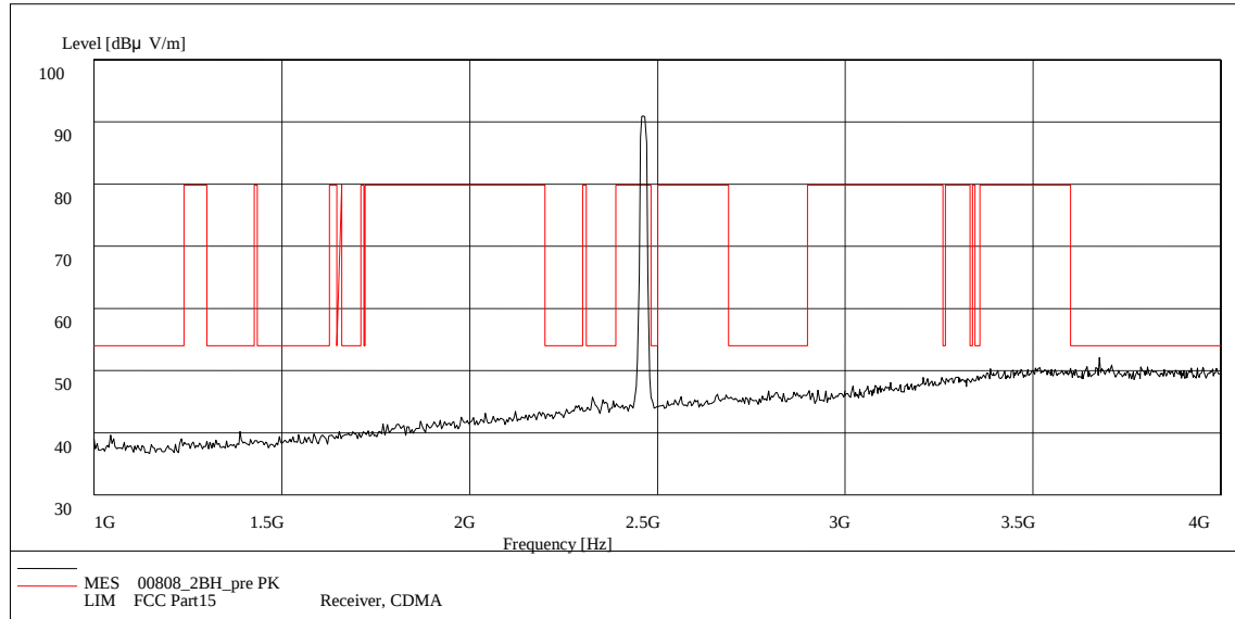
Fig. 74 Radiated Spurious Emission (802.11b, Ch11, 1 GHz-4 GHz)
