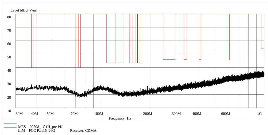
Fig. 84 Radiated Spurious Emission (802.11g, Ch11, 30 MHz-1 GHz)
