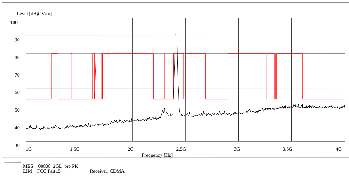
Fig. 78 Radiated Spurious Emission (802.11g, Ch1, 1 GHz-4 GHz)
