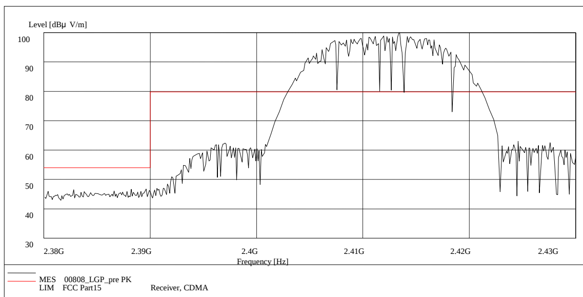
Fig. 76 Radiated Spurious Emission (Power): 802.11g, ch1, 2.38 GHz - 2.43GHz
