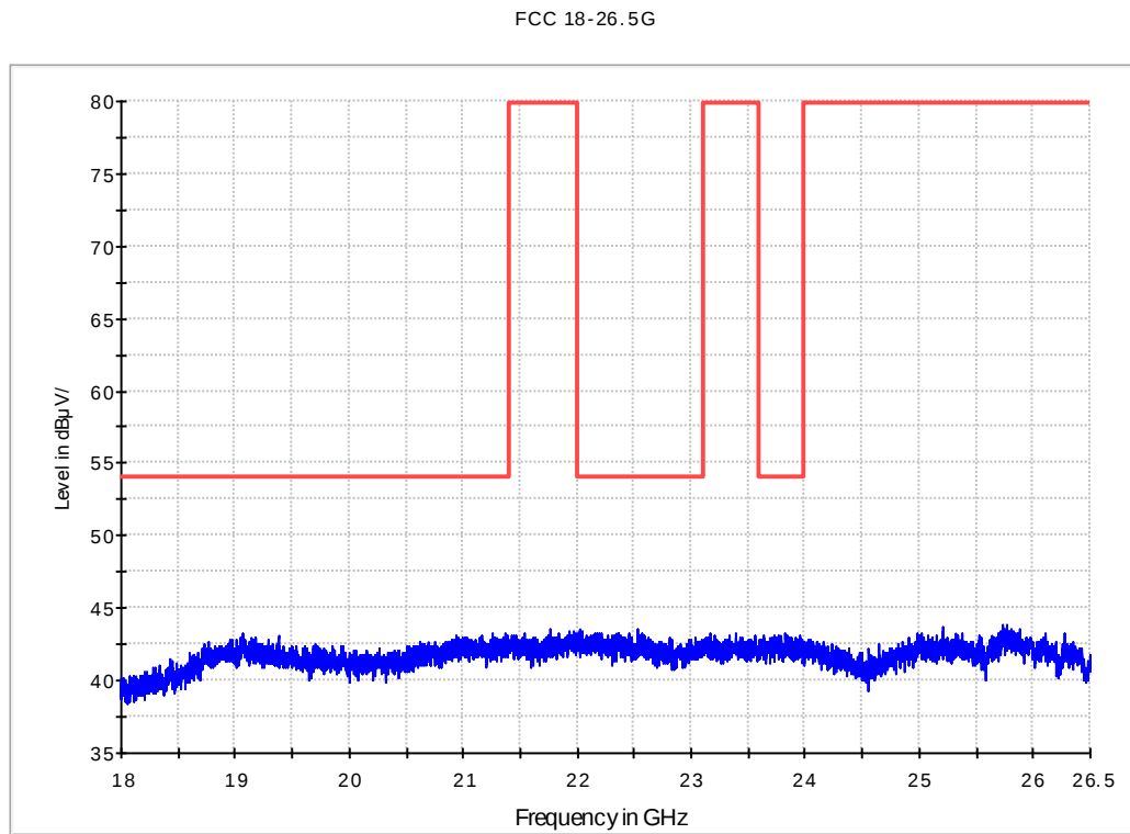
Fig. 87 Radiated emission: 18 GHz - 26.5 GHz
