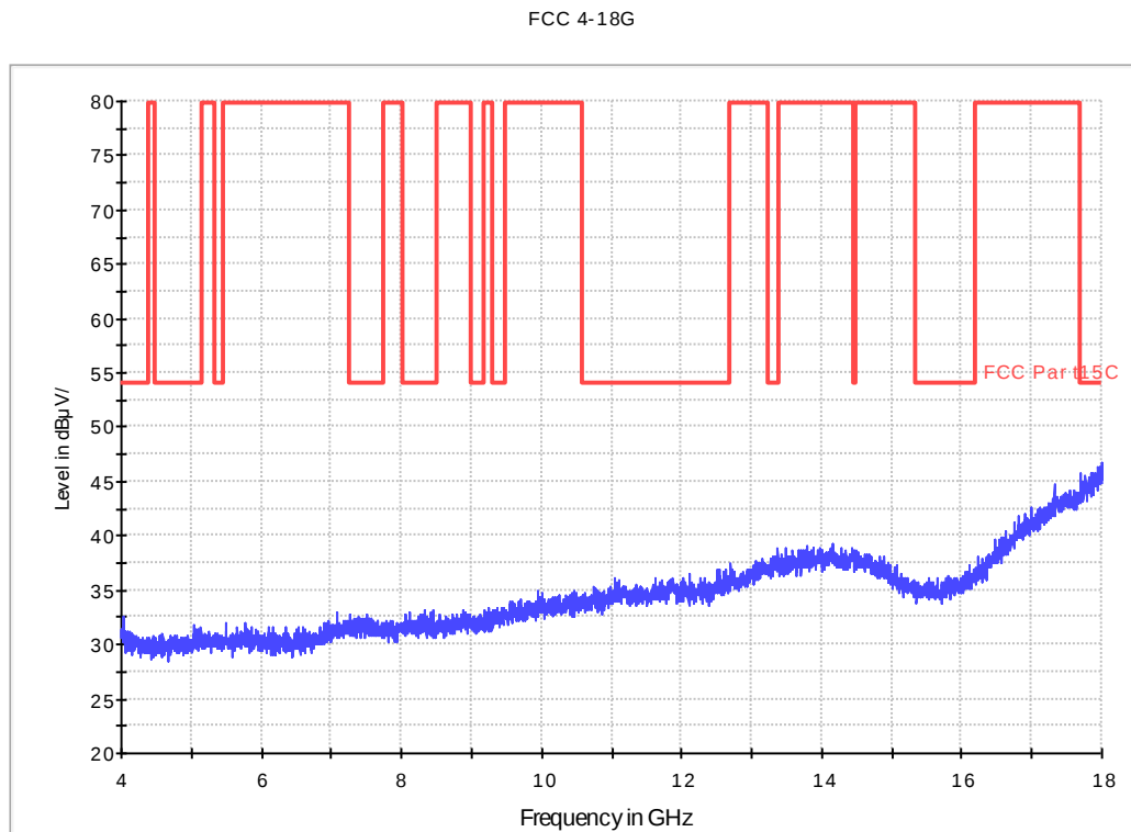
Fig. 71 Radiated Spurious Emission (802.11b, Ch6, 4 GHz-18 GHz)
