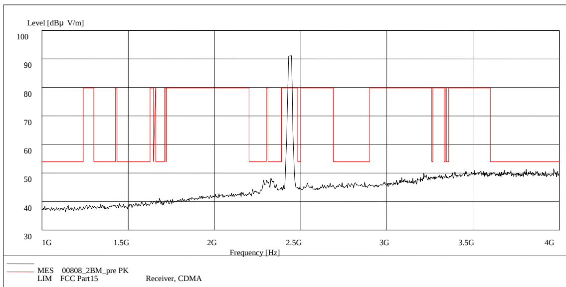
Fig. 70 Radiated Spurious Emission (802.11b, Ch6, 1 GHz-4 GHz)
