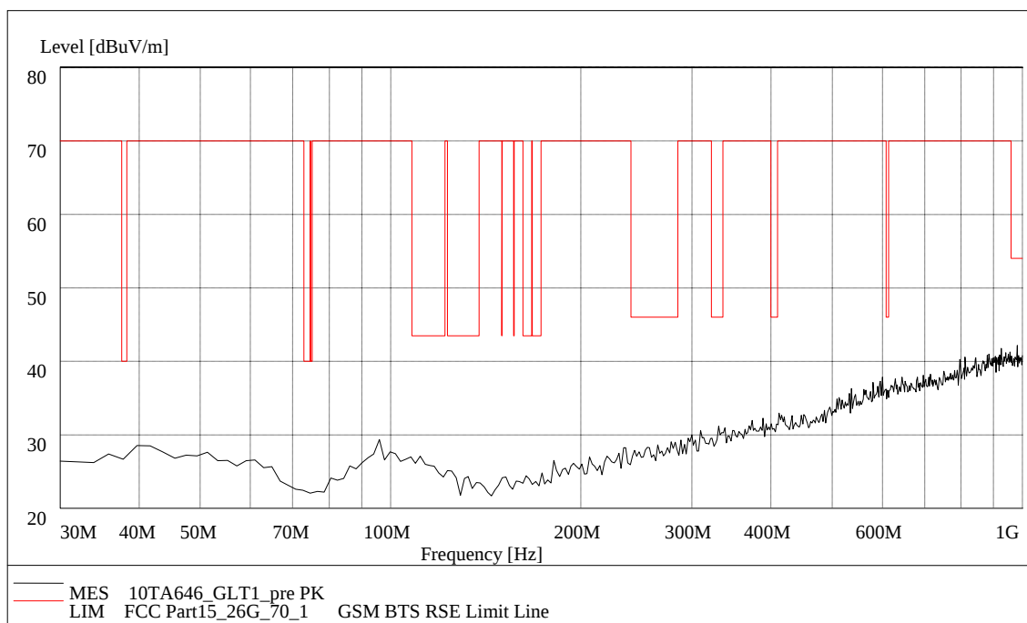
Fig. 46 Radiated Spurious Emission (802.11g, Ch1, 30 MHz-1 GHz)
