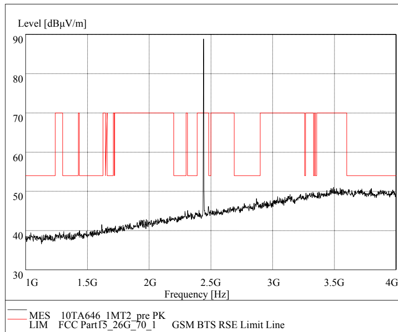
Fig. 44 Radiated emission: GFSK, Channel 39, 1 GHz - 4 GHz
