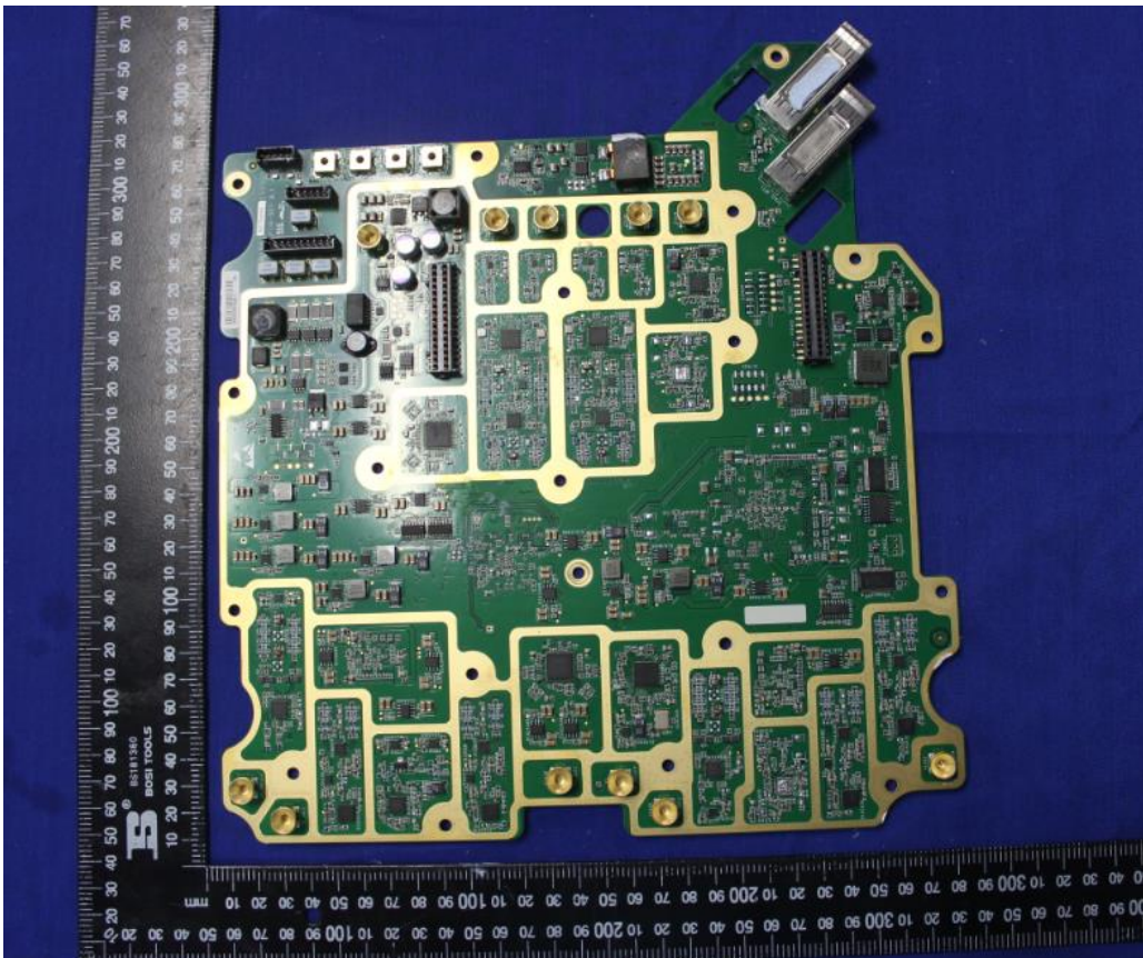
The Top view of R61TAA26A board
