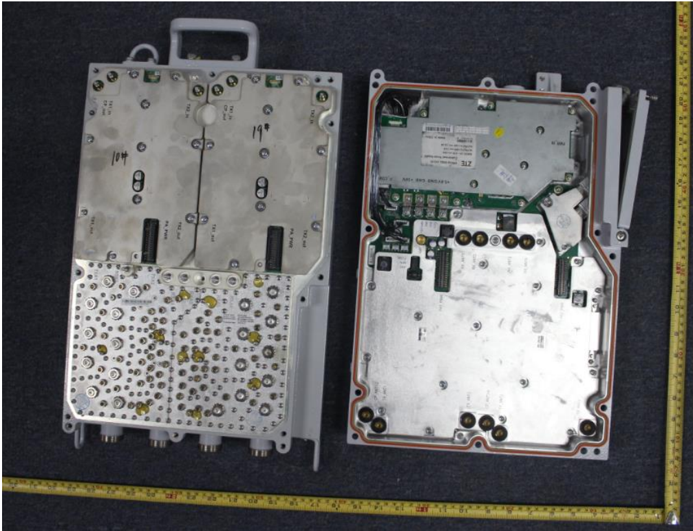
The Internal view of ZXSDR R8854 S2600
