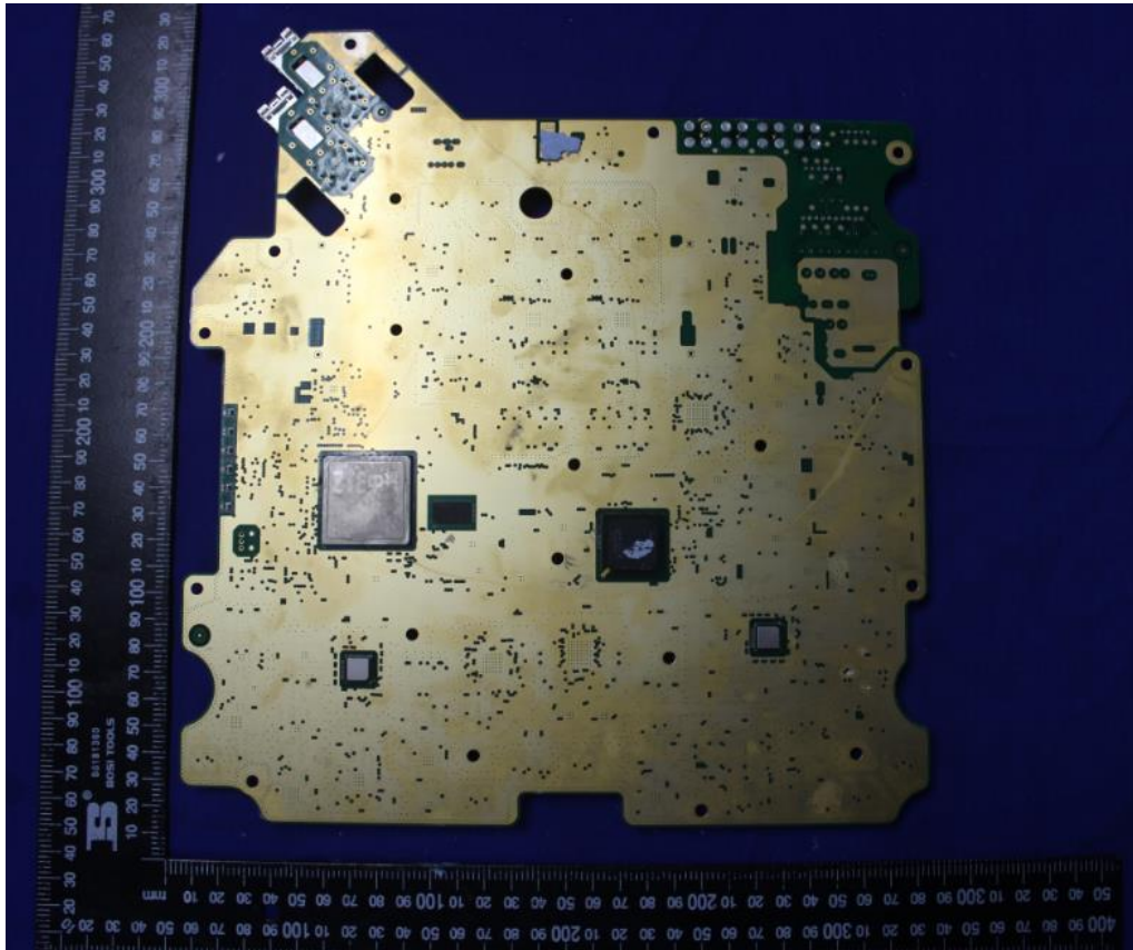
The Bottom view of R61TAA26A board
