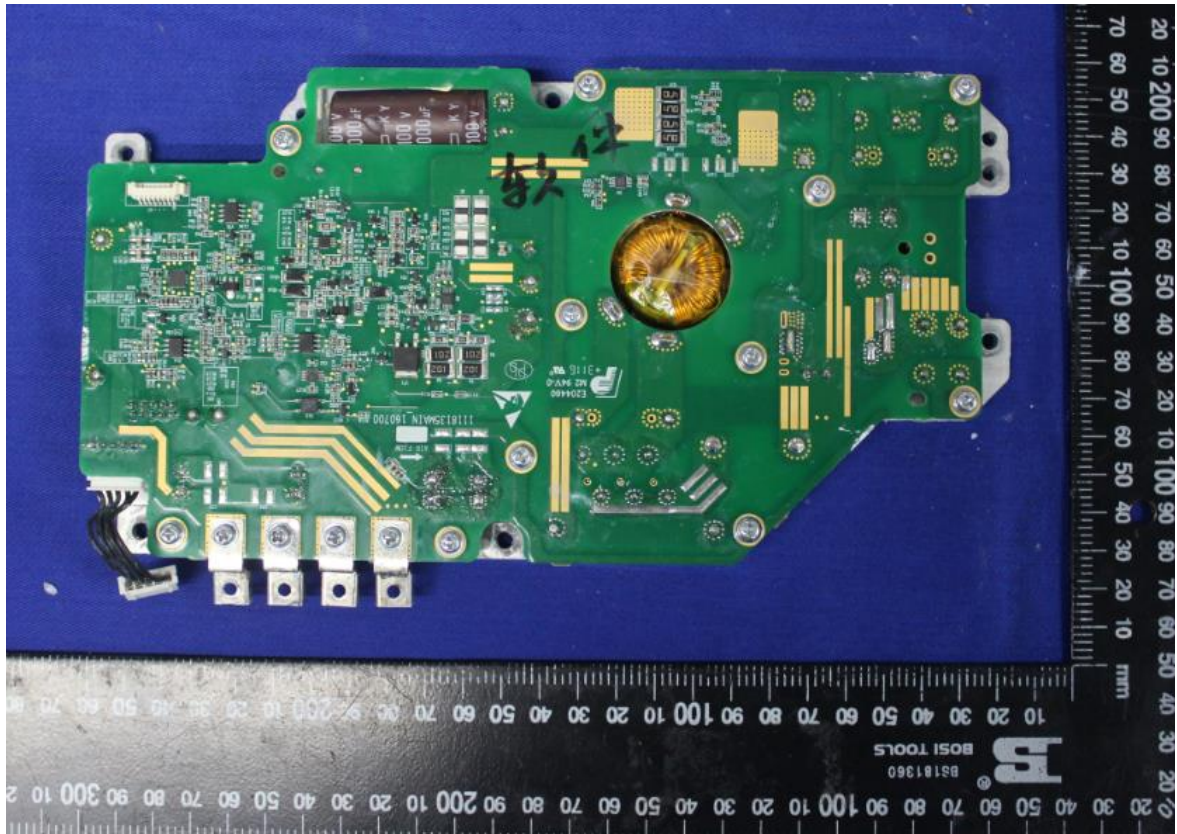
The internal view of PPC32 D021
