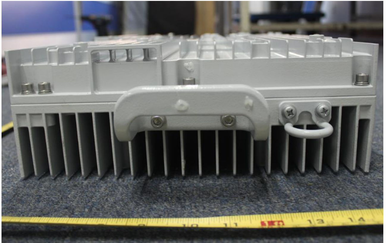
The sideview of ZXSDR R8854 S2600
