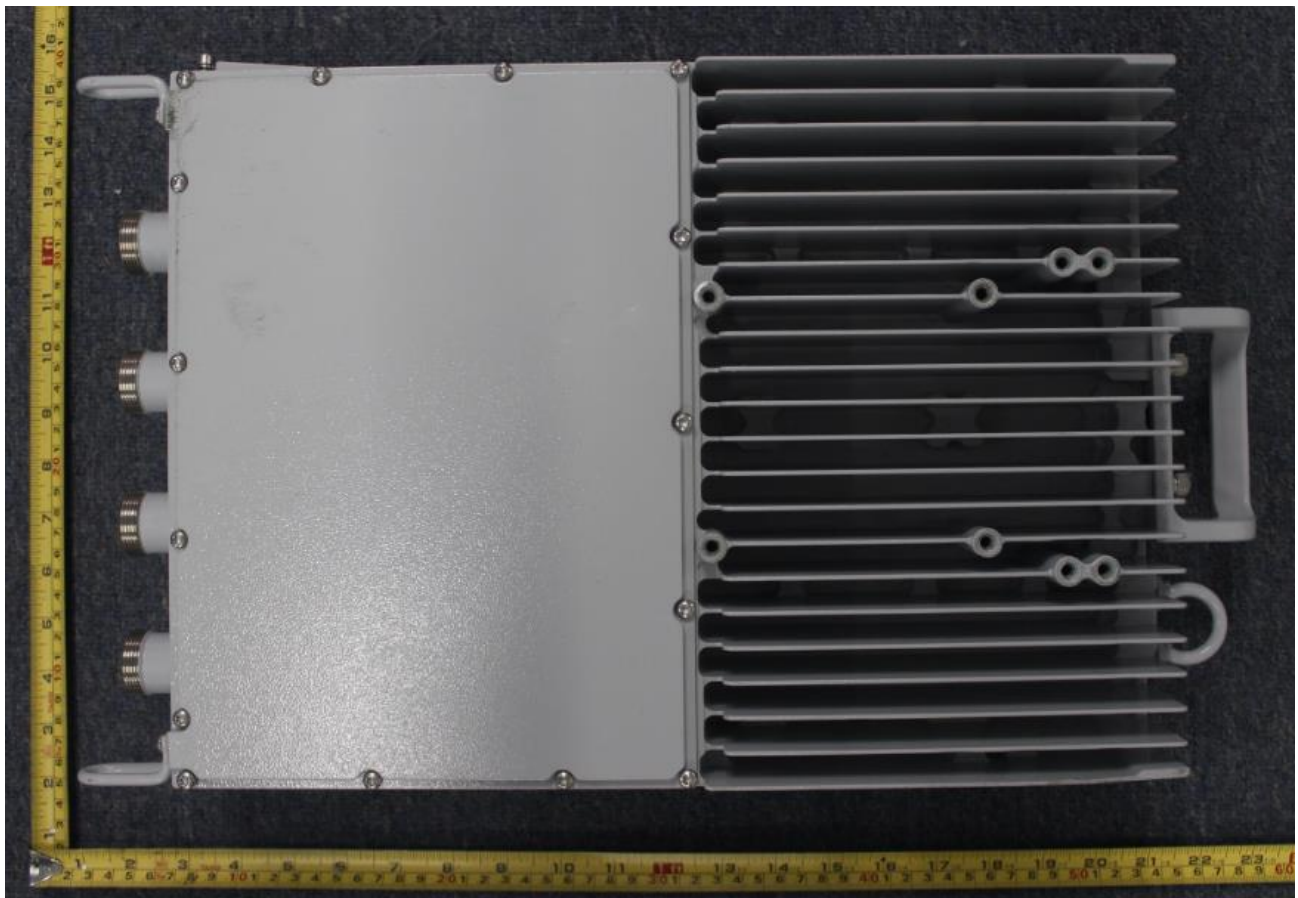
The sideview of ZXSDR R8854 S2600
