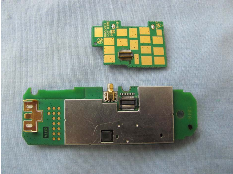
Pic A-11 USB Modem Disassembly
