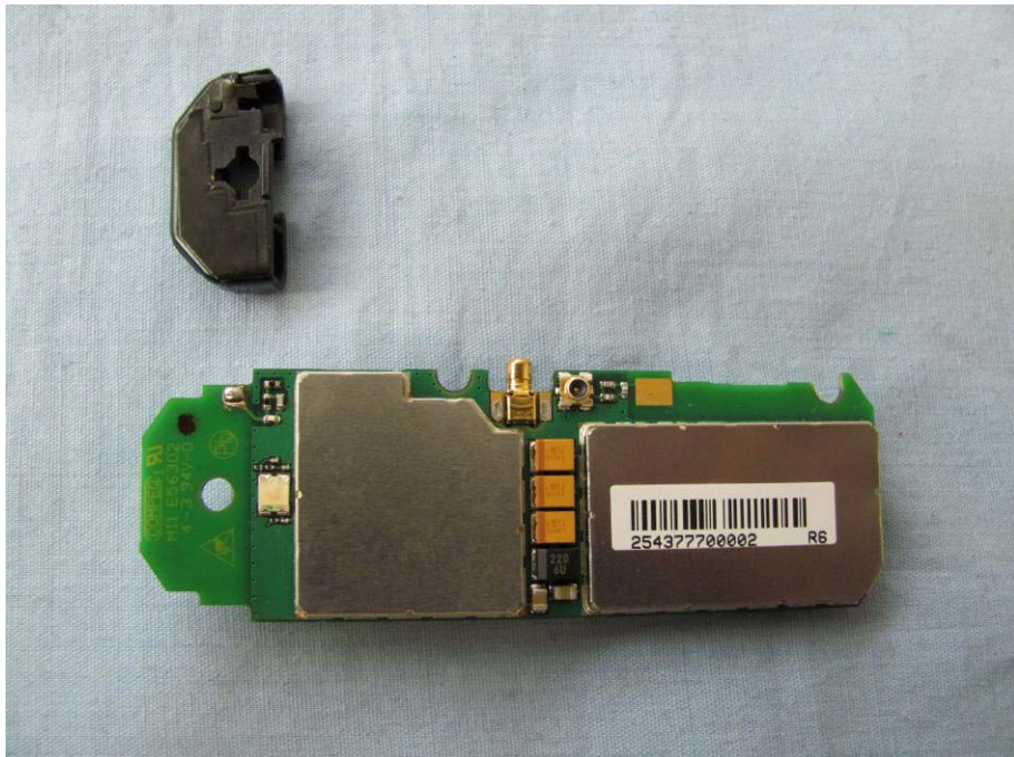
Pic A-10 USB Modem Disassembly
