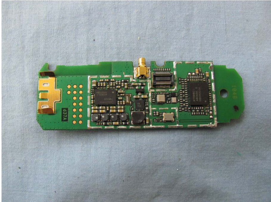
Pic A-13 USB Modem Disassembly
