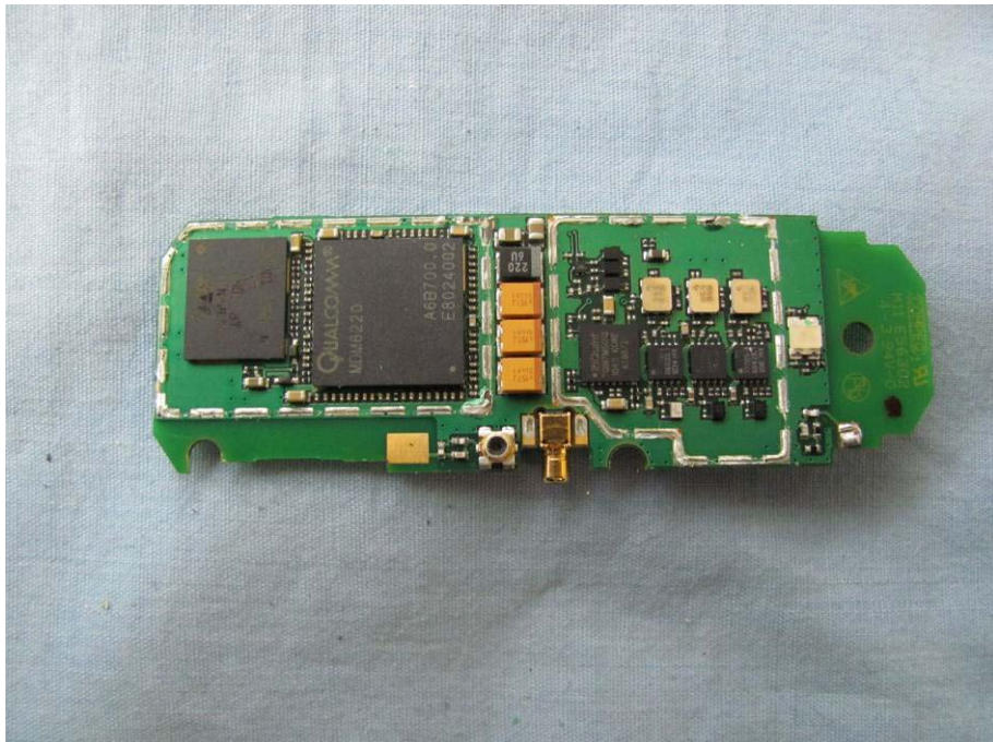
Pic A-12 USB Modem Disassembly
