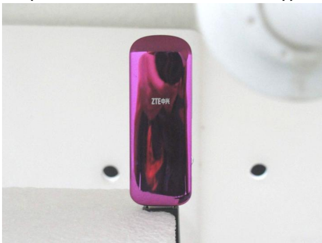
USB Cable Plug-in for USB Tip Mode (Tip Mode with Phantom 0.5 cm Gap)
