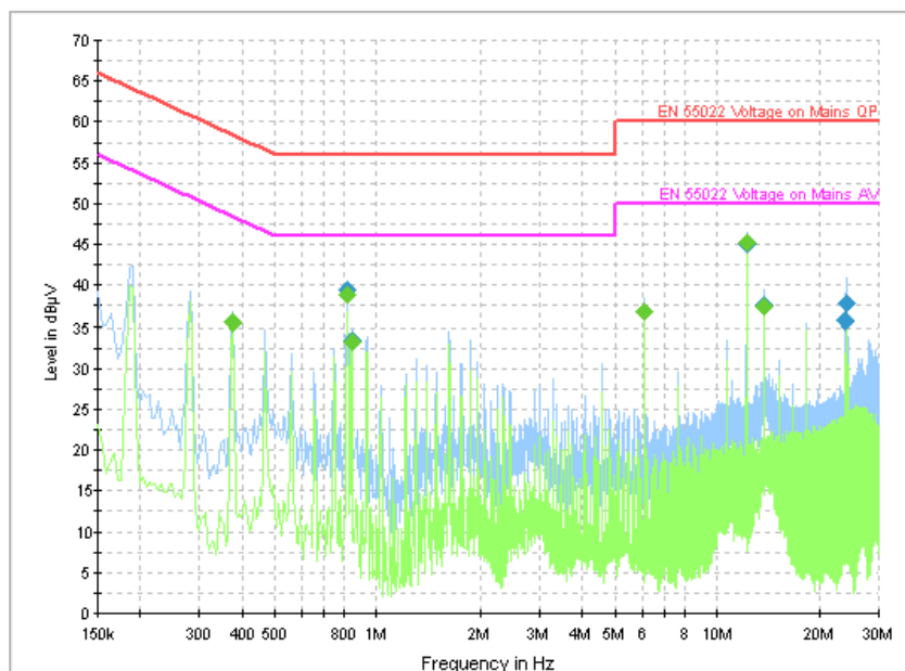
Figure A.4 Conducted Emission
