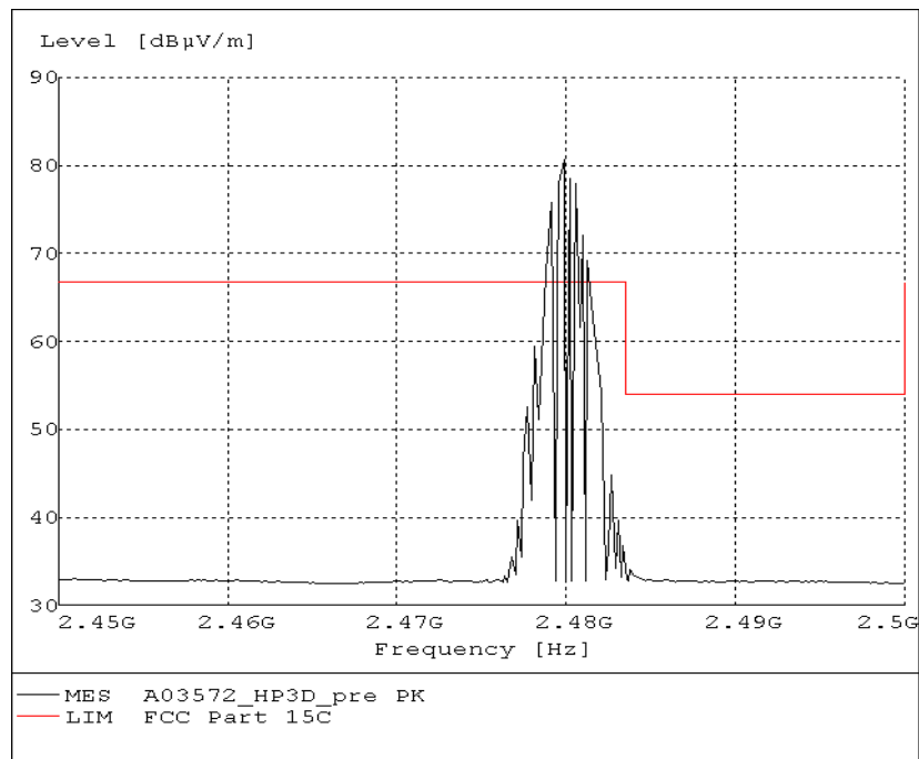
Fig.92. Radiated emission (Power): 8DPSK, high channel
