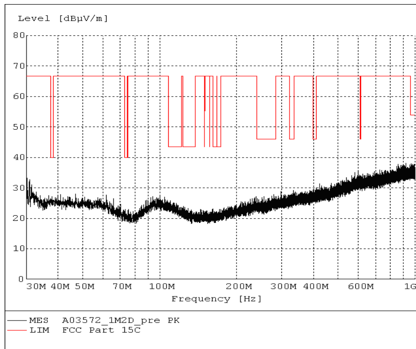
Fig.73. Radiated emission: \pi/4 DQPSK, Channel 39, 30 MHz - 1 GHz
