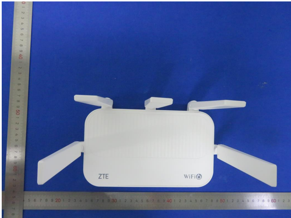
View 1#
