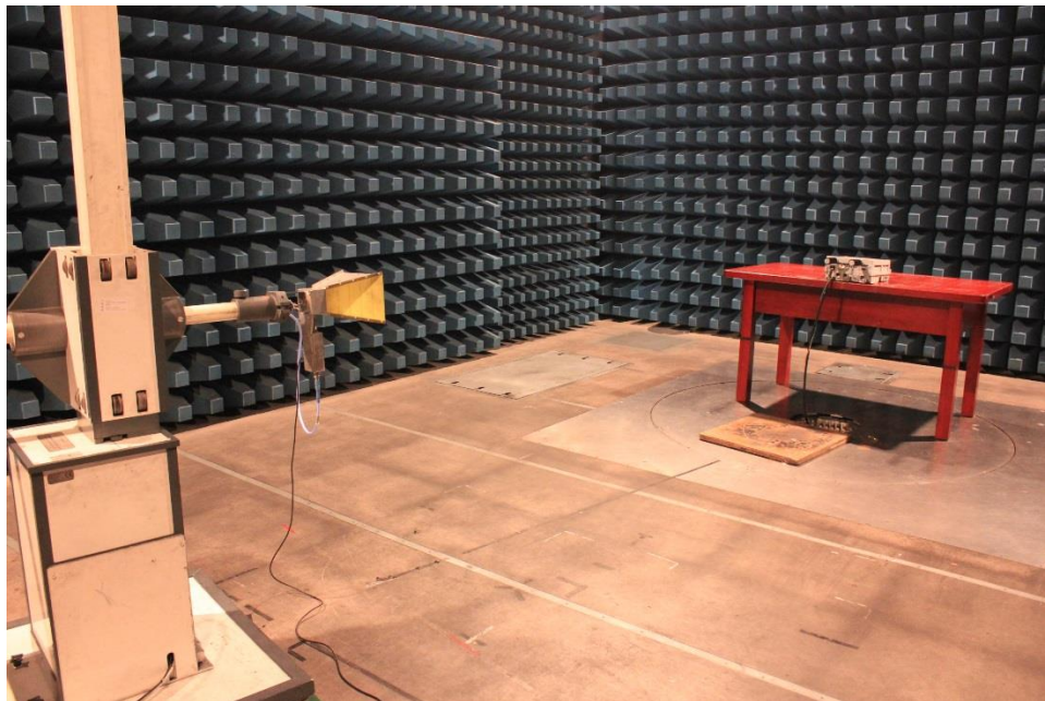
Radiated spurious emission (Above 1GHz)
