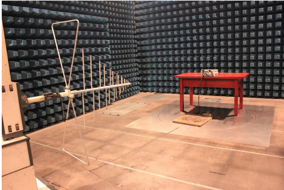
Radiated spurious emission (below 1GHz)
