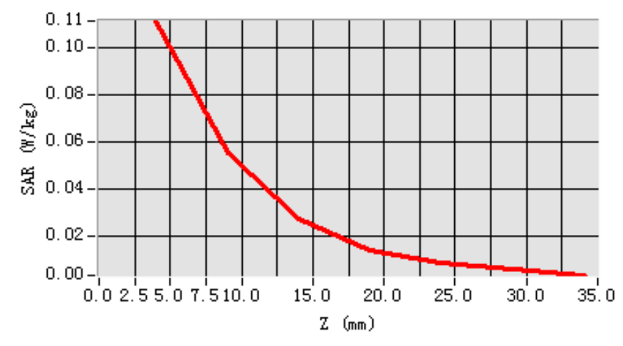
SAR, Z Axis Scan (X = -30, Y = 9)
