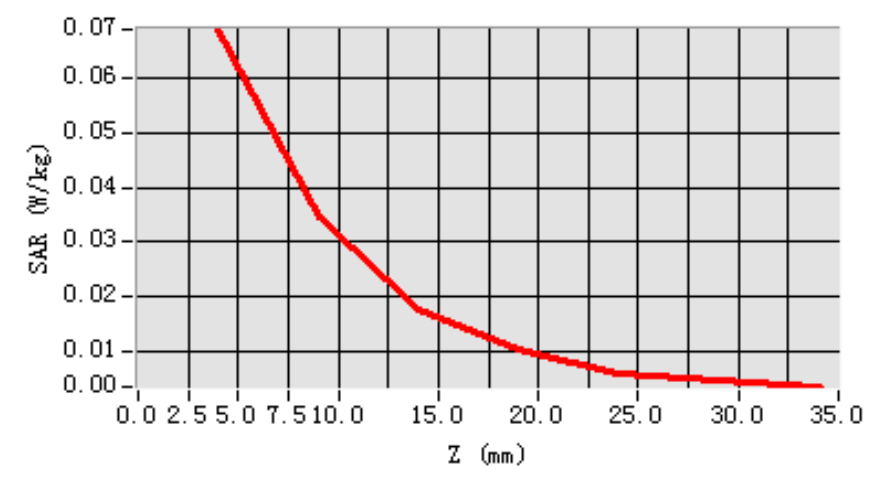
SAR, Z Axis Scan (X = -31, Y = 5)
