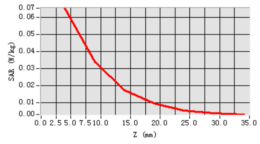
SAR, Z Axis Scan (X = -34, Y = -1)
