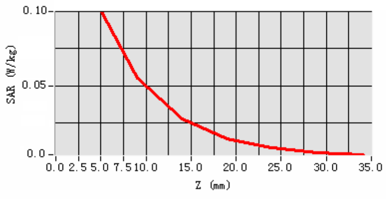
SAR, Z Axis Scan (X = -25, Y = 1)
