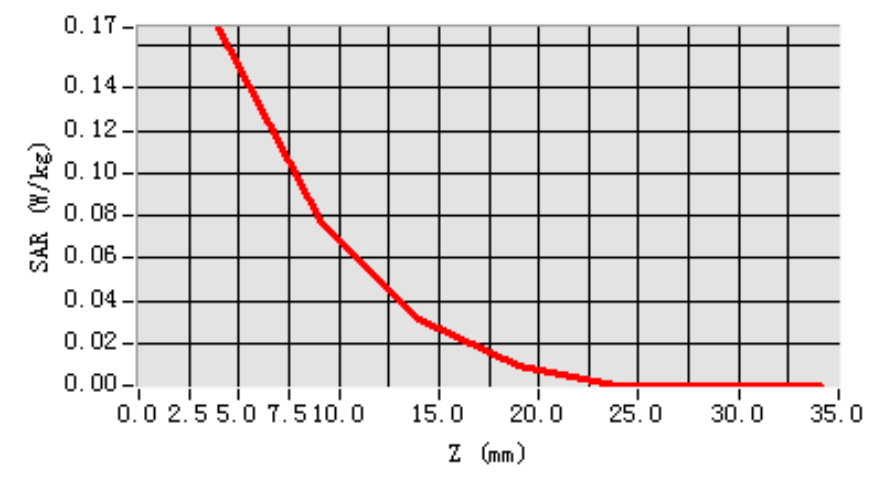
SAR, Z Axis Scan (X = 0, Y = -3)
