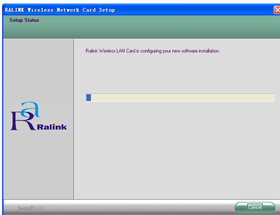
Figure 2-2 Start Setup
