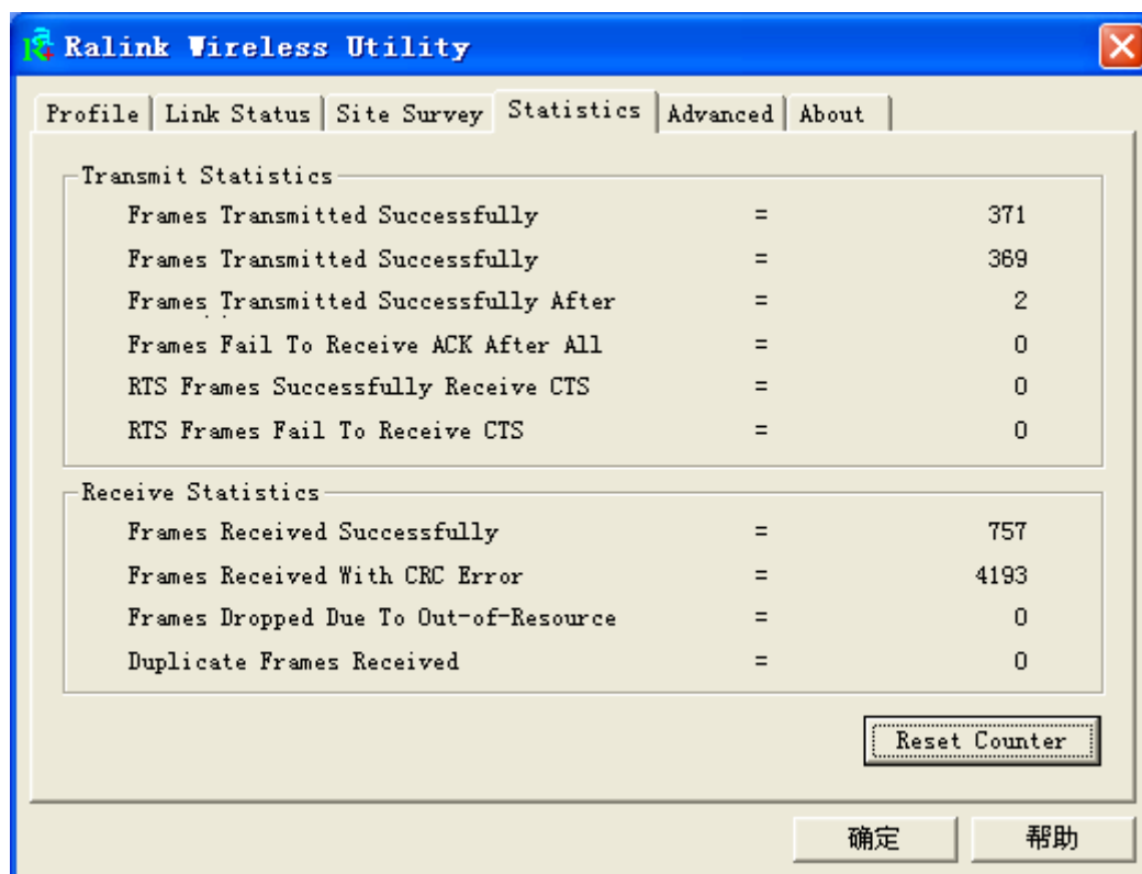
Figure 3-6 Statistics tab
