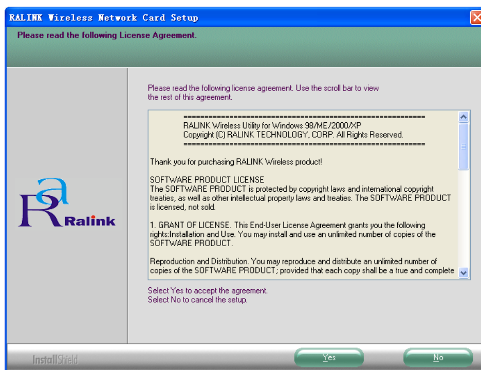
Figure 2-1 Preparing Setup
