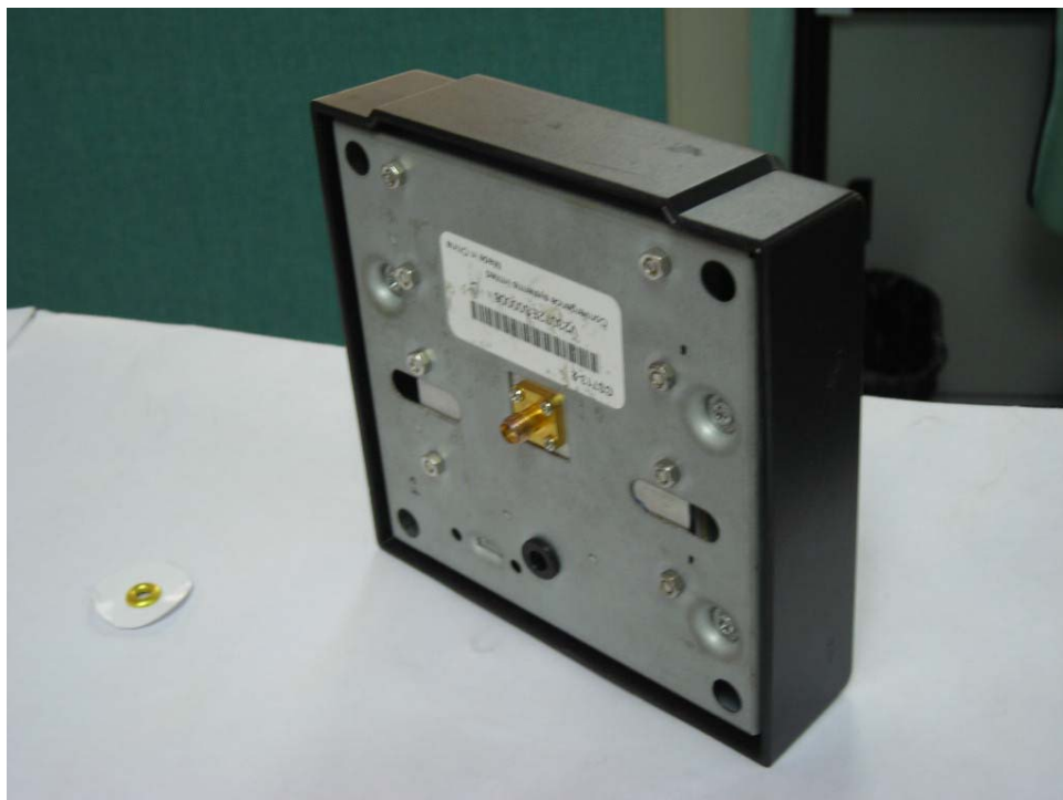
Antenna for Radiated Emission Test
