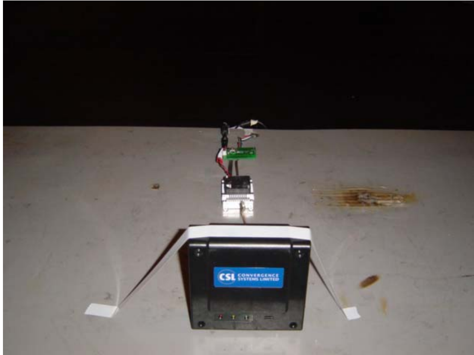
Test Setup of Radiated Emission Test
