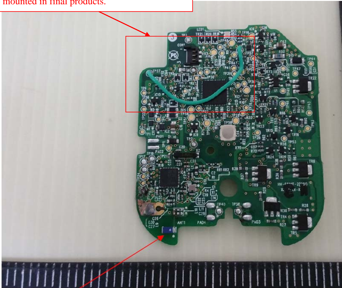
Chip Antenna
