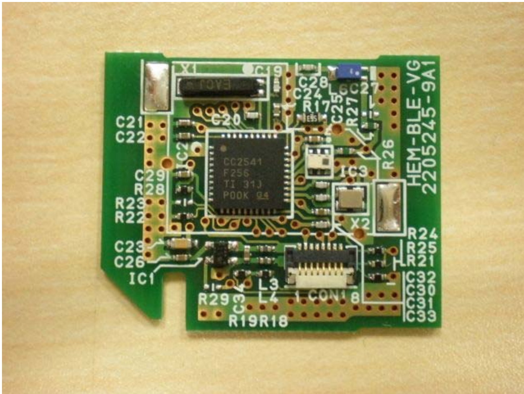
Top Side (w/o Shielding)
