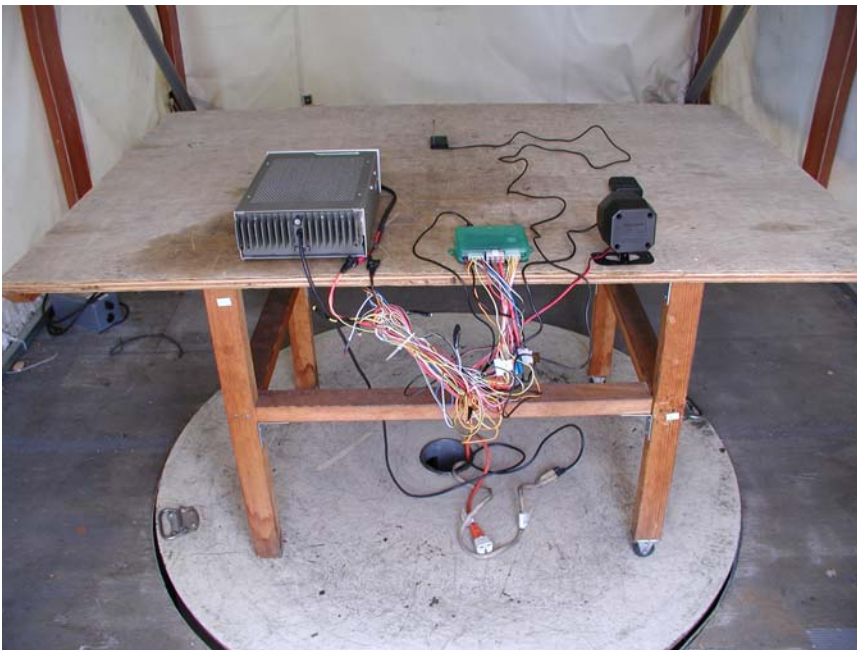
Radiated Emission Photograph – Rear View
