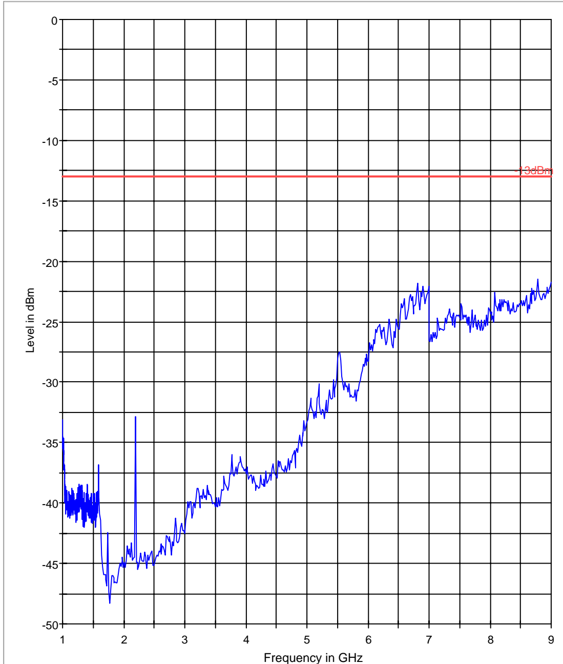
FCC 22 1-9GHz
