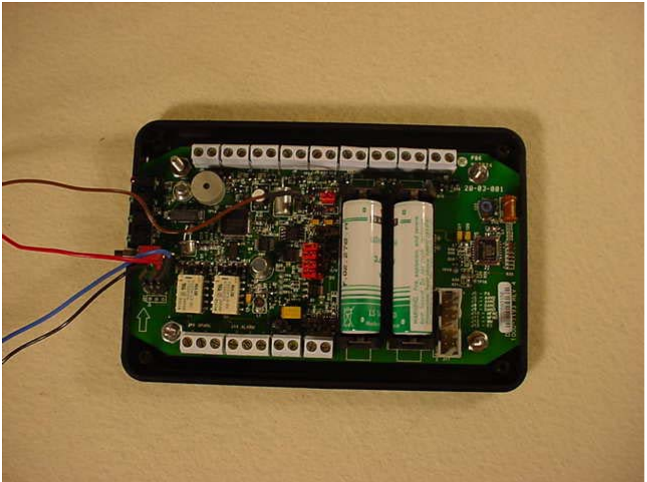
Figure 3: Test Setup - Overhead
