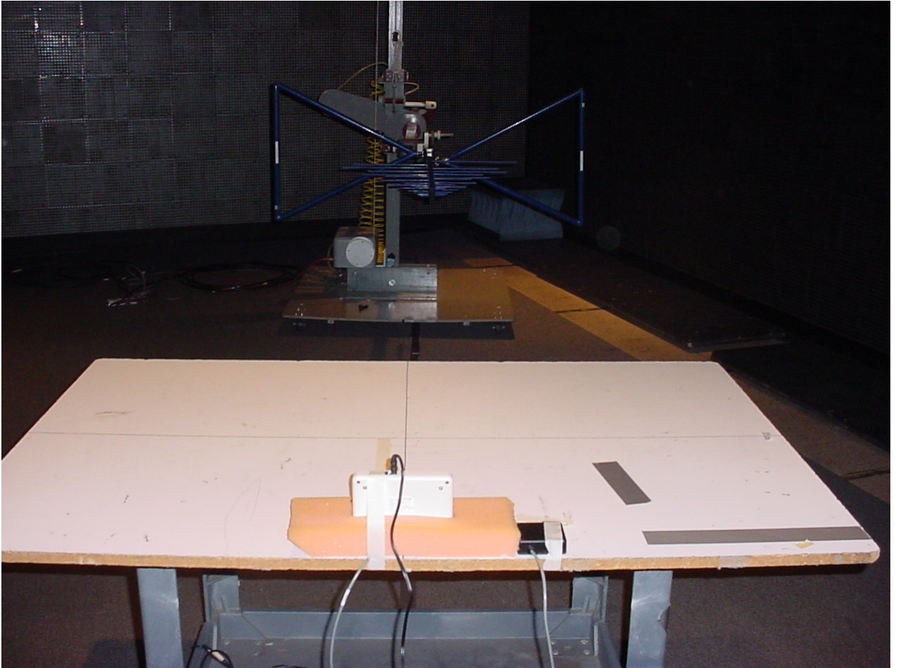
Figure 1: Radiated Emissions – Below 1GHz
