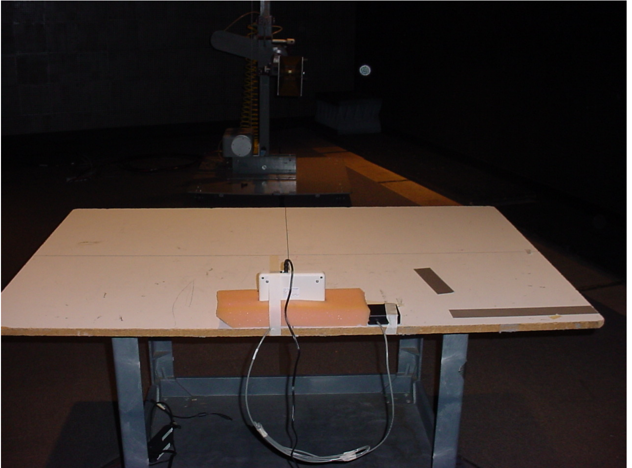
Figure 3: Radiated Emissions – Above 1GHz
