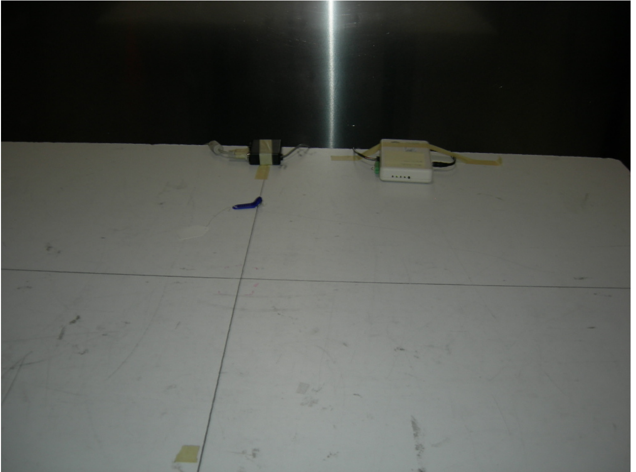
Figure 5: Conducted Emissions
