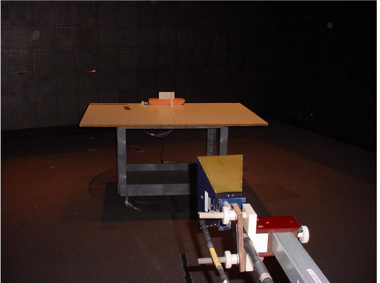
Figure 4: Radiated Emissions – Above 1GHz
